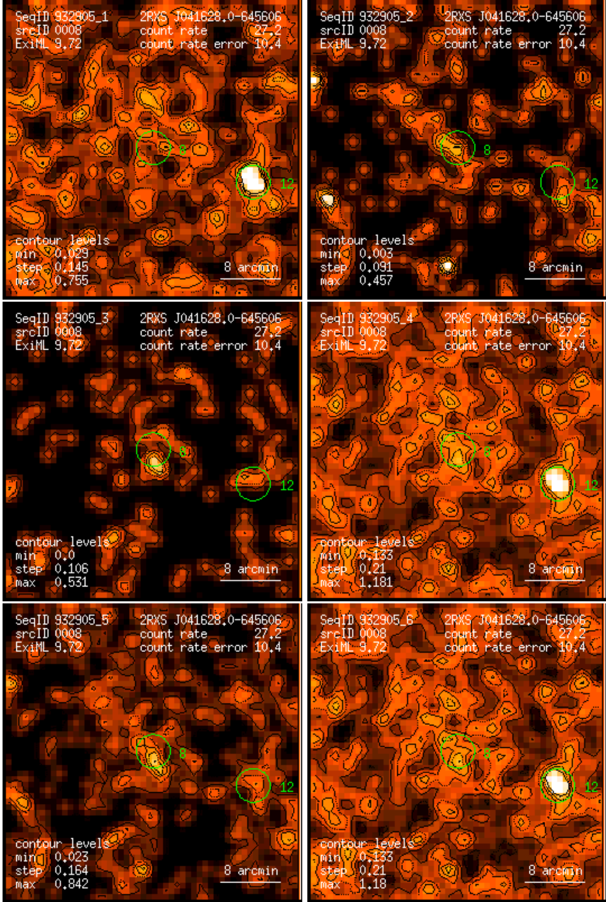
Figure 8: RASS 932905: detection 0008: band rate images, Gaussian filter: (1) PSPC channels 11 – 41, (2) 52 – 90, (3) 91 – 201, (4) 11 – 235, (5) 52 – 201, (6) 11 – 201. Broad band rates in counts/ks. Band rate contour levels in counts/ks/arcmin 2 .
