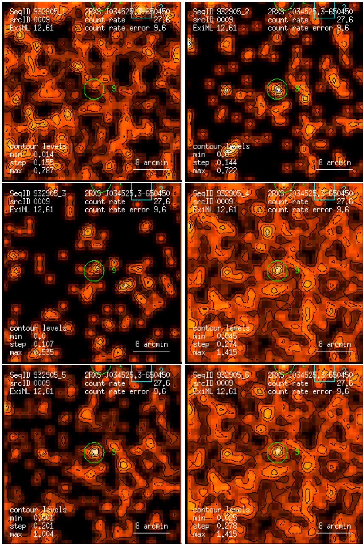
Figure 9: RASS 932905: detection 0009: band rate images, Gaussian filter: (1) PSPC channels 11 – 41, (2) 52 – 90, (3) 91 – 201, (4) 11 – 235, (5) 52 – 201, (6) 11 – 201. Broad band rates in counts/ks. Band rate contour levels in counts/ks/arcmin 2 .
