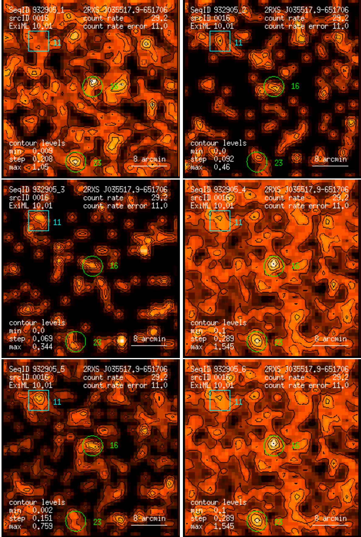
Figure 16: RASS 932905: detection 0016: band rate images, Gaussian filter: (1) PSPC channels 11 – 41, (2) 52 – 90, (3) 91 – 201, (4) 11 – 235, (5) 52 – 201, (6) 11 – 201. Broad band rates in counts/ks. Band rate contour levels in counts/ks/arcmin 2 .
