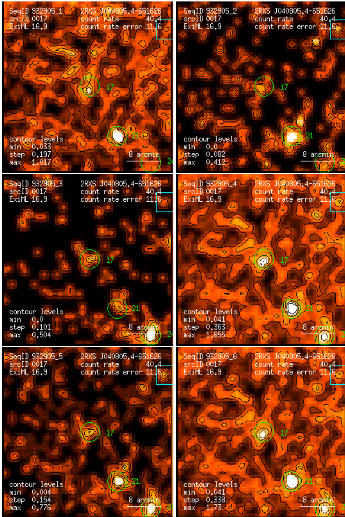
Figure 17: RASS 932905: detection 0017: band rate images, Gaussian filter: (1) PSPC channels 11 – 41, (2) 52 – 90, (3) 91 – 201, (4) 11 – 235, (5) 52 – 201, (6) 11 – 201. Broad band rates in counts/ks. Band rate contour levels in counts/ks/arcmin 2 .
