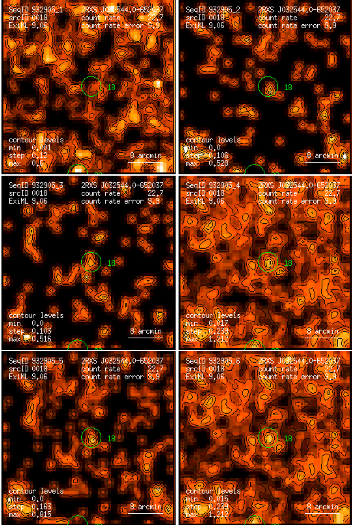
Figure 18: RASS 932905: detection 0018: band rate images, Gaussian filter: (1) PSPC channels 11 – 41, (2) 52 – 90, (3) 91 – 201, (4) 11 – 235, (5) 52 – 201, (6) 11 – 201. Broad band rates in counts/ks. Band rate contour levels in counts/ks/arcmin 2 .
