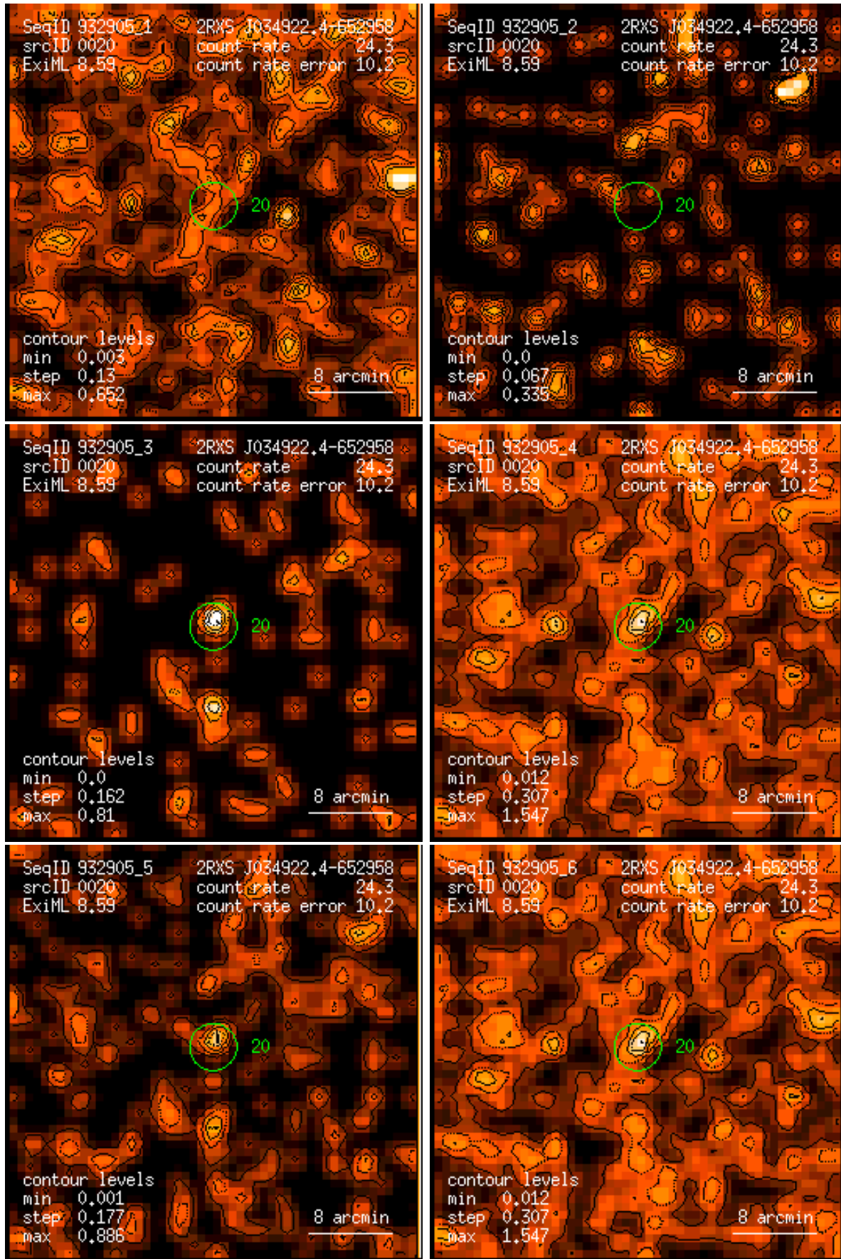
Figure 20: RASS 932905: detection 0020: band rate images, Gaussian filter: (1) PSPC channels 11 – 41, (2) 52 – 90, (3) 91 – 201, (4) 11 – 235, (5) 52 – 201, (6) 11 – 201. Broad band rates in counts/ks. Band rate contour levels in counts/ks/arcmin 2 .
