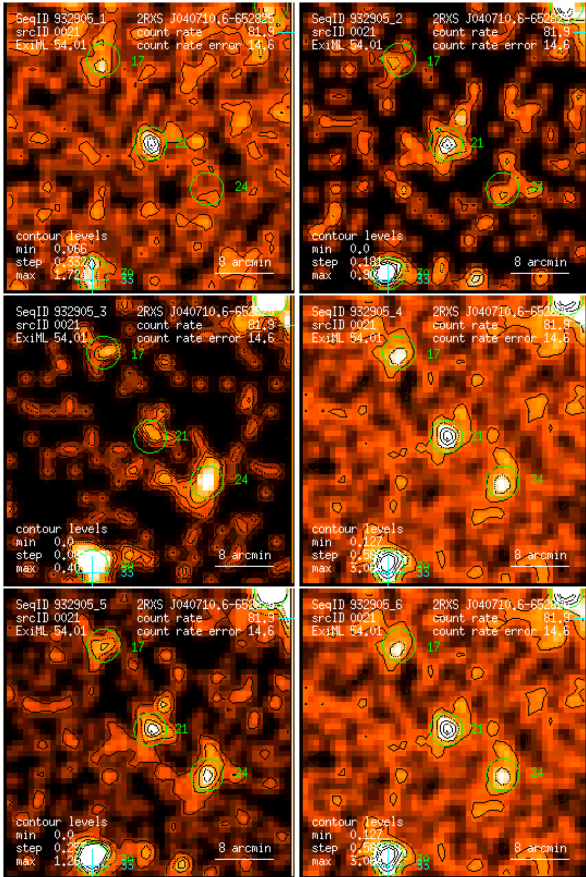
Figure 21: RASS 932905: detection 0021: band rate images, Gaussian filter: (1) PSPC channels 11 – 41, (2) 52 – 90, (3) 91 – 201, (4) 11 – 235, (5) 52 – 201, (6) 11 – 201. Broad band rates in counts/ks. Band rate contour levels in counts/ks/arcmin 2 .
