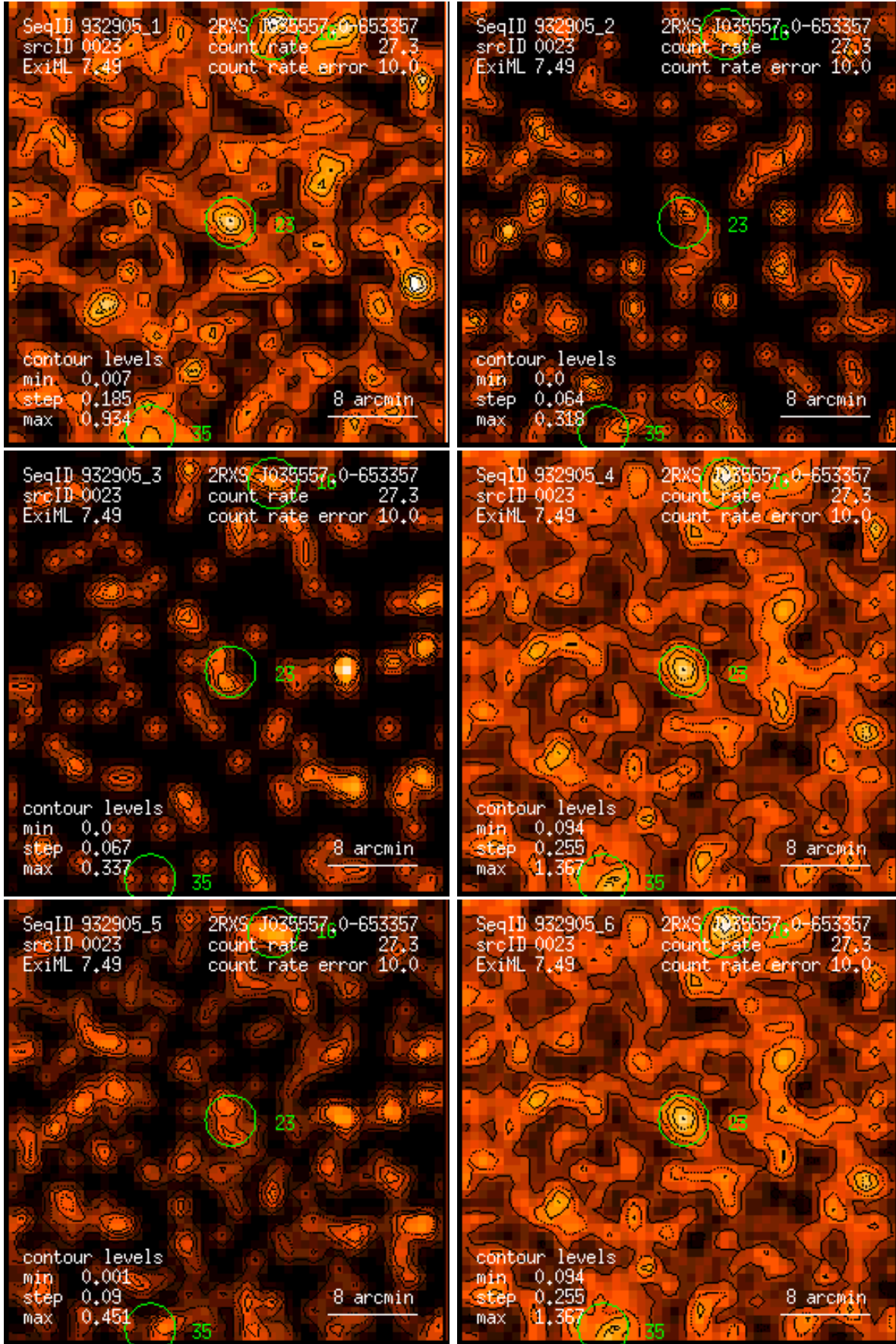
Figure 23: RASS 932905: detection 0023: band rate images, Gaussian filter: (1) PSPC channels 11 – 41, (2) 52 – 90, (3) 91 – 201, (4) 11 – 235, (5) 52 – 201, (6) 11 – 201. Broad band rates in counts/ks. Band rate contour levels in counts/ks/arcmin 2 .
