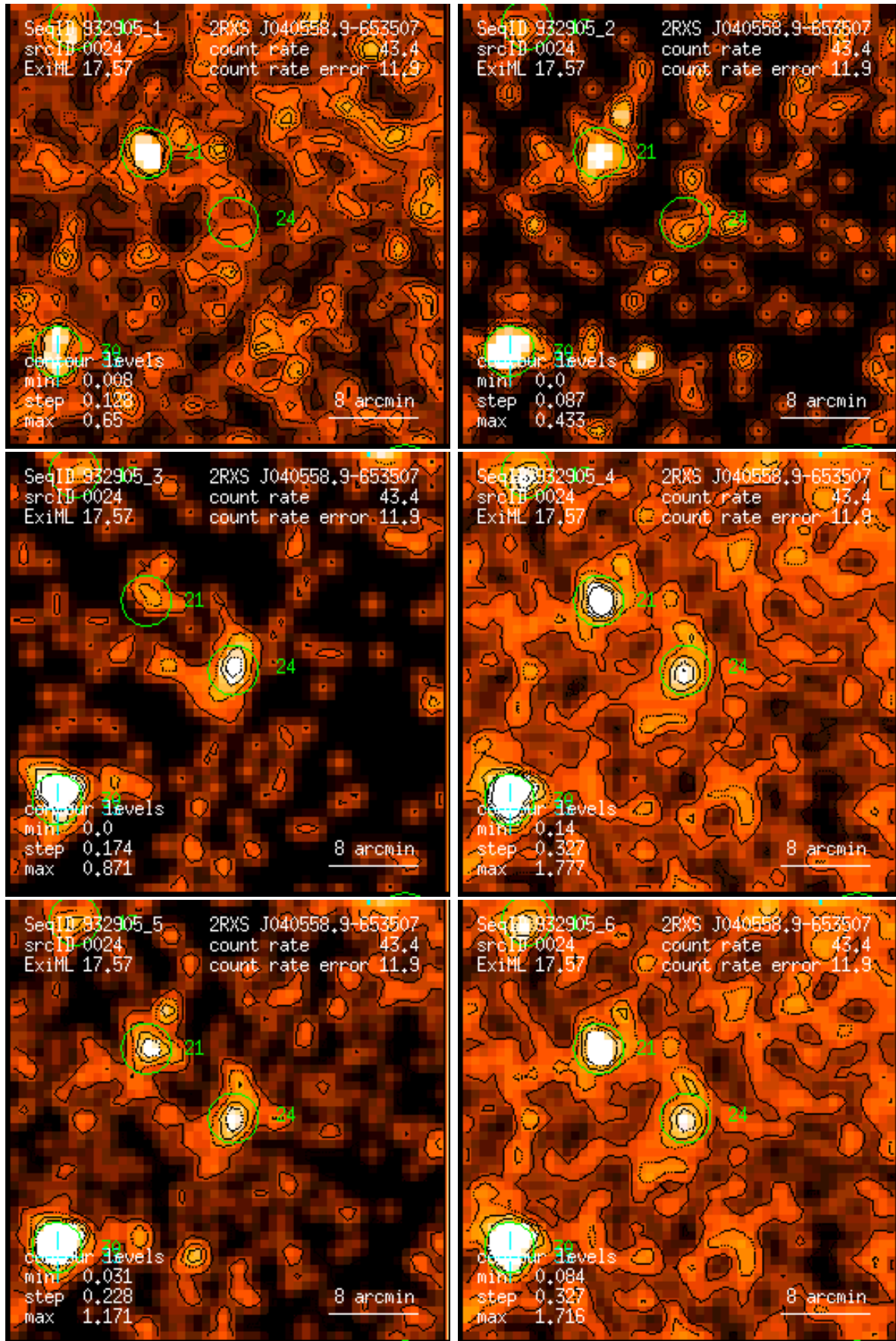
Figure 24: RASS 932905: detection 0024: band rate images, Gaussian filter: (1) PSPC channels 11 – 41, (2) 52 – 90, (3) 91 – 201, (4) 11 – 235, (5) 52 – 201, (6) 11 – 201. Broad band rates in counts/ks. Band rate contour levels in counts/ks/arcmin 2 .
