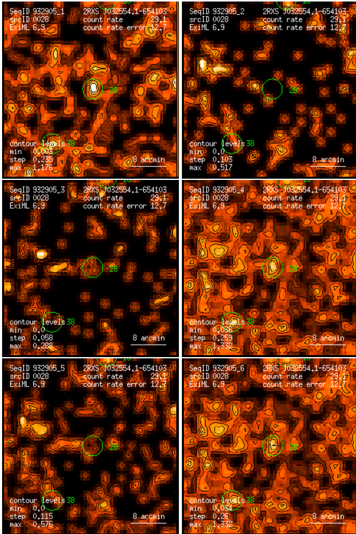
Figure 28: RASS 932905: detection 0028: band rate images, Gaussian filter: (1) PSPC channels 11 – 41, (2) 52 – 90, (3) 91 – 201, (4) 11 – 235, (5) 52 – 201, (6) 11 – 201. Broad band rates in counts/ks. Band rate contour levels in counts/ks/arcmin 2 .
