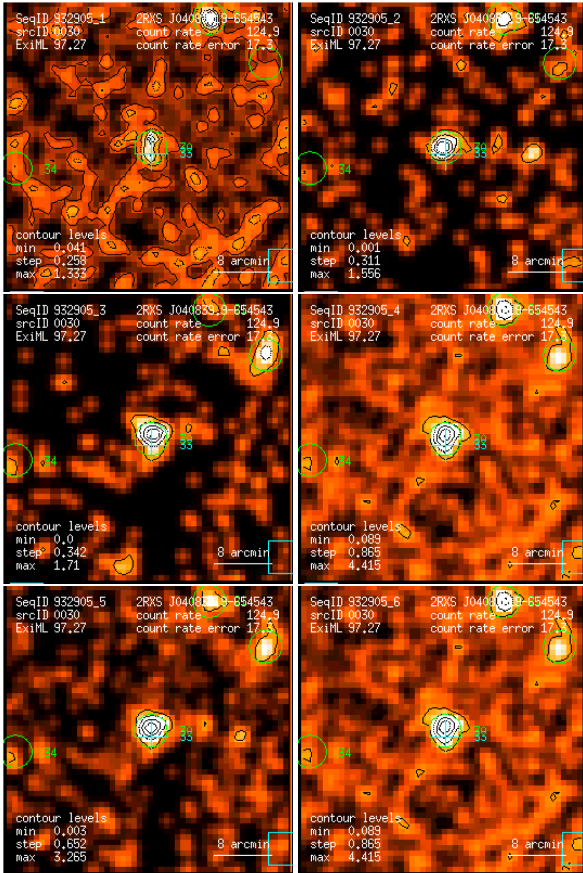
Figure 30: RASS 932905: detection 0030: band rate images, Gaussian filter: (1) PSPC channels 11 – 41, (2) 52 – 90, (3) 91 – 201, (4) 11 – 235, (5) 52 – 201, (6) 11 – 201. Broad band rates in counts/ks. Band rate contour levels in counts/ks/arcmin 2 .
