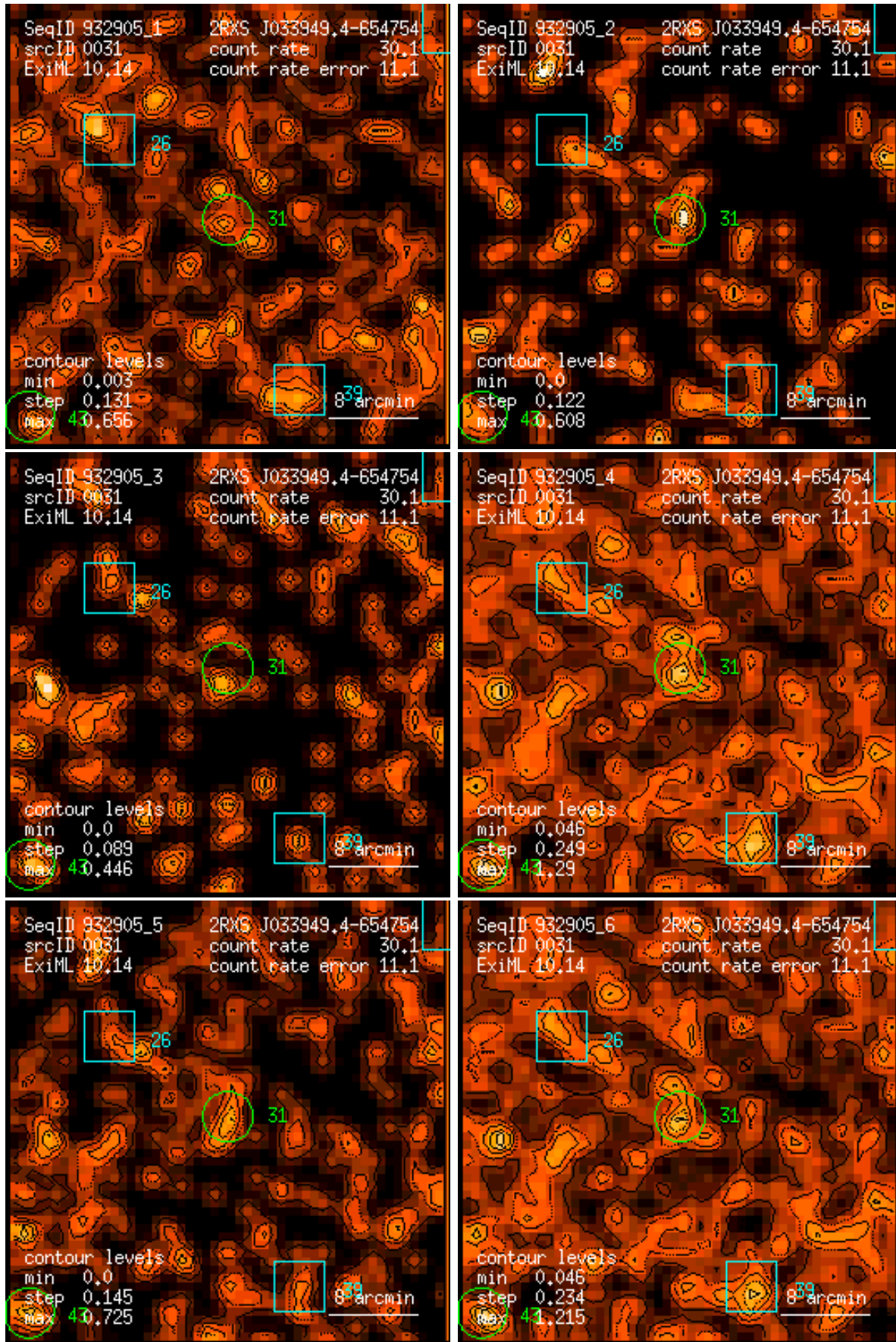
Figure 31: RASS 932905: detection 0031: band rate images, Gaussian filter: (1) PSPC channels 11 – 41, (2) 52 – 90, (3) 91 – 201, (4) 11 – 235, (5) 52 – 201, (6) 11 – 201. Broad band rates in counts/ks. Band rate contour levels in counts/ks/arcmin 2 .
