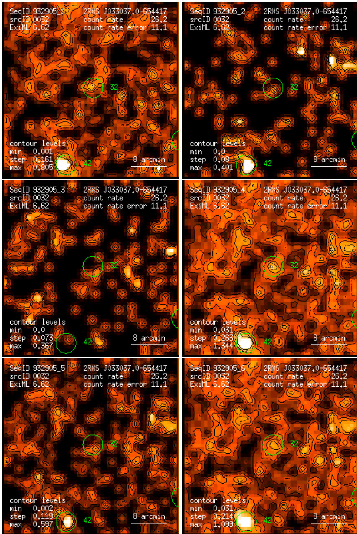
Figure 32: RASS 932905: detection 0032: band rate images, Gaussian filter: (1) PSPC channels 11 – 41, (2) 52 – 90, (3) 91 – 201, (4) 11 – 235, (5) 52 – 201, (6) 11 – 201. Broad band rates in counts/ks. Band rate contour levels in counts/ks/arcmin 2 .
