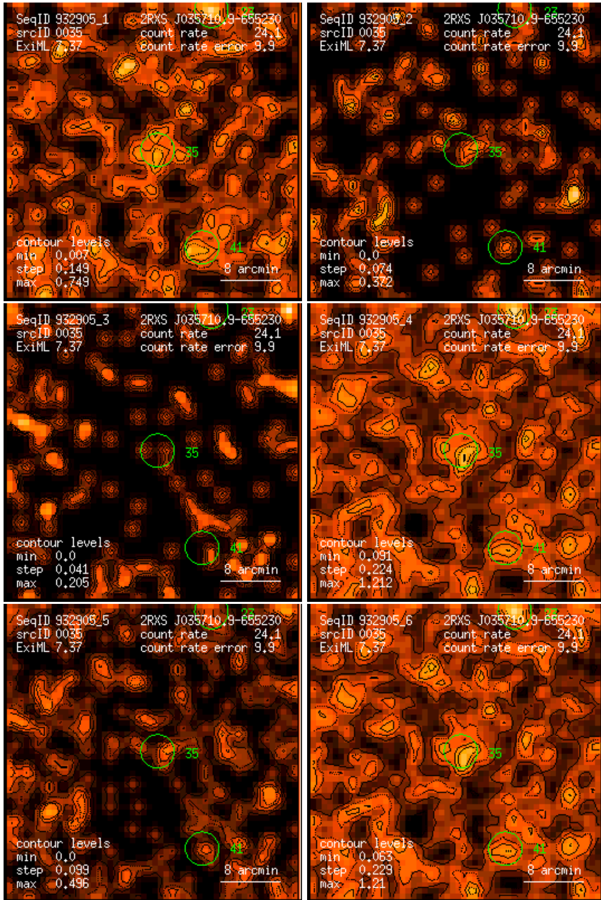
Figure 35: RASS 932905: detection 0035: band rate images, Gaussian filter: (1) PSPC channels 11 – 41, (2) 52 – 90, (3) 91 – 201, (4) 11 – 235, (5) 52 – 201, (6) 11 – 201. Broad band rates in counts/ks. Band rate contour levels in counts/ks/arcmin 2 .
