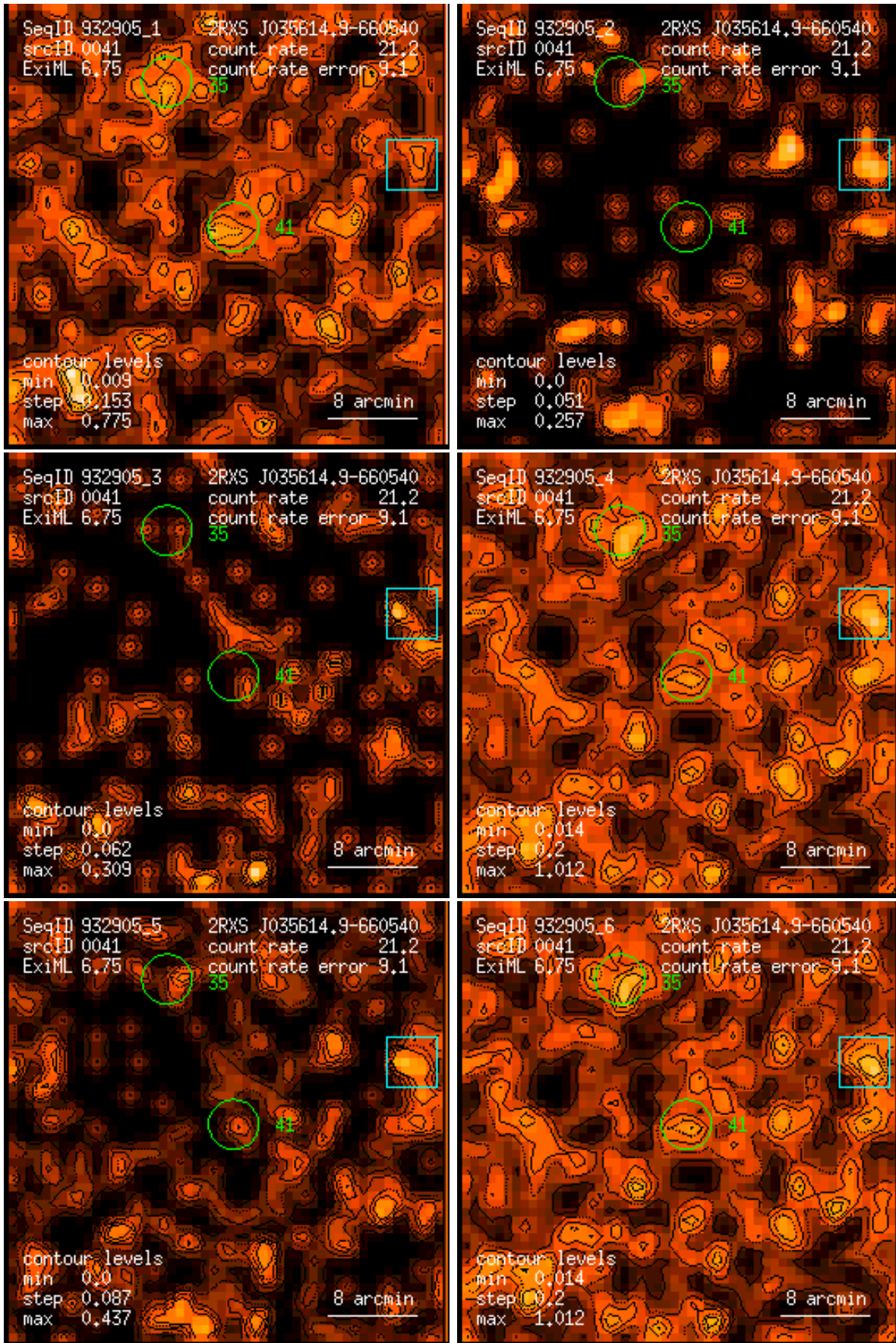
Figure 41: RASS 932905: detection 0041: band rate images, Gaussian filter: (1) PSPC channels 11 – 41, (2) 52 – 90, (3) 91 – 201, (4) 11 – 235, (5) 52 – 201, (6) 11 – 201. Broad band rates in counts/ks. Band rate contour levels in counts/ks/arcmin 2 .
