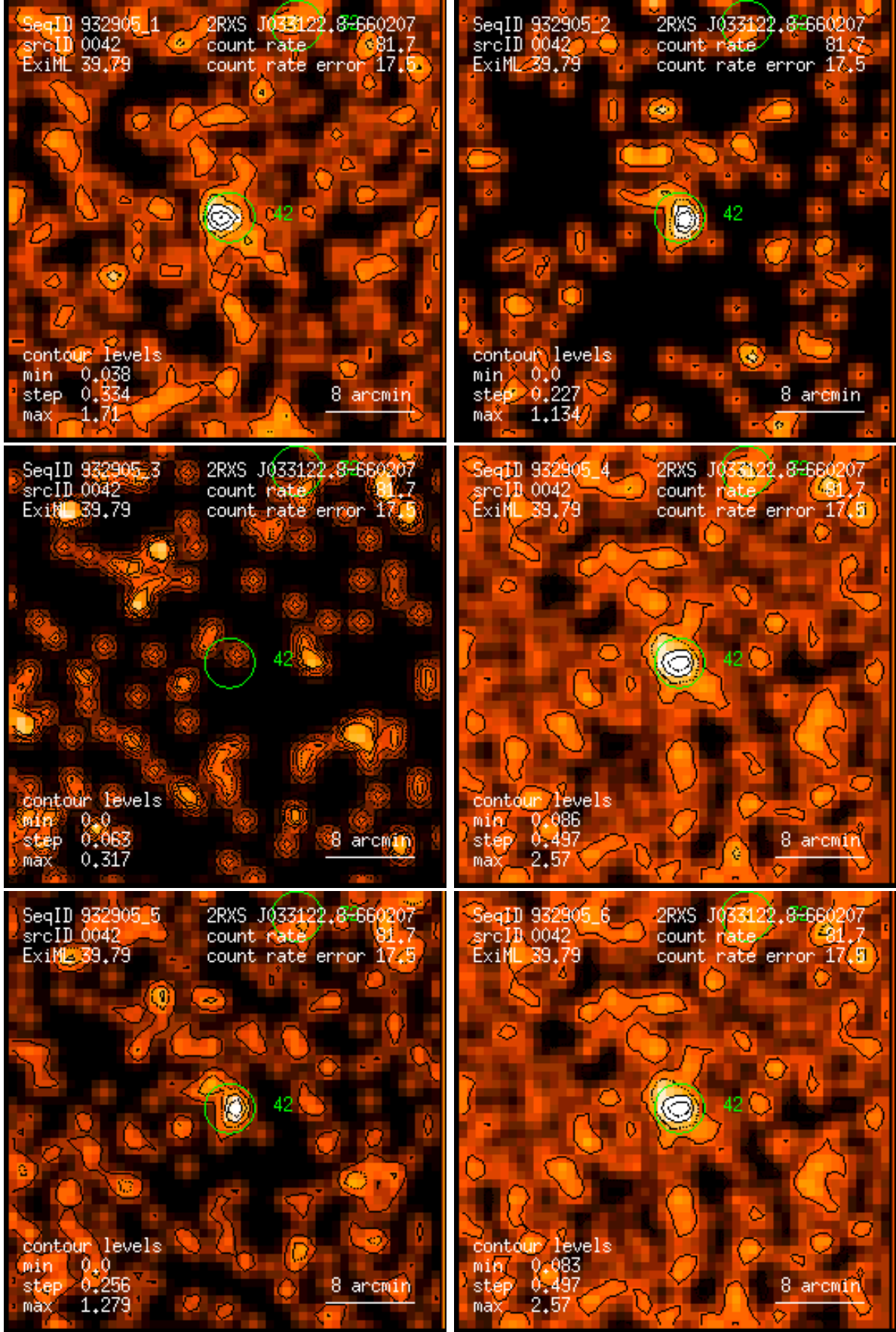
Figure 42: RASS 932905: detection 0042: band rate images, Gaussian filter: (1) PSPC channels 11 – 41, (2) 52 – 90, (3) 91 – 201, (4) 11 – 235, (5) 52 – 201, (6) 11 – 201. Broad band rates in counts/ks. Band rate contour levels in counts/ks/arcmin 2 .
