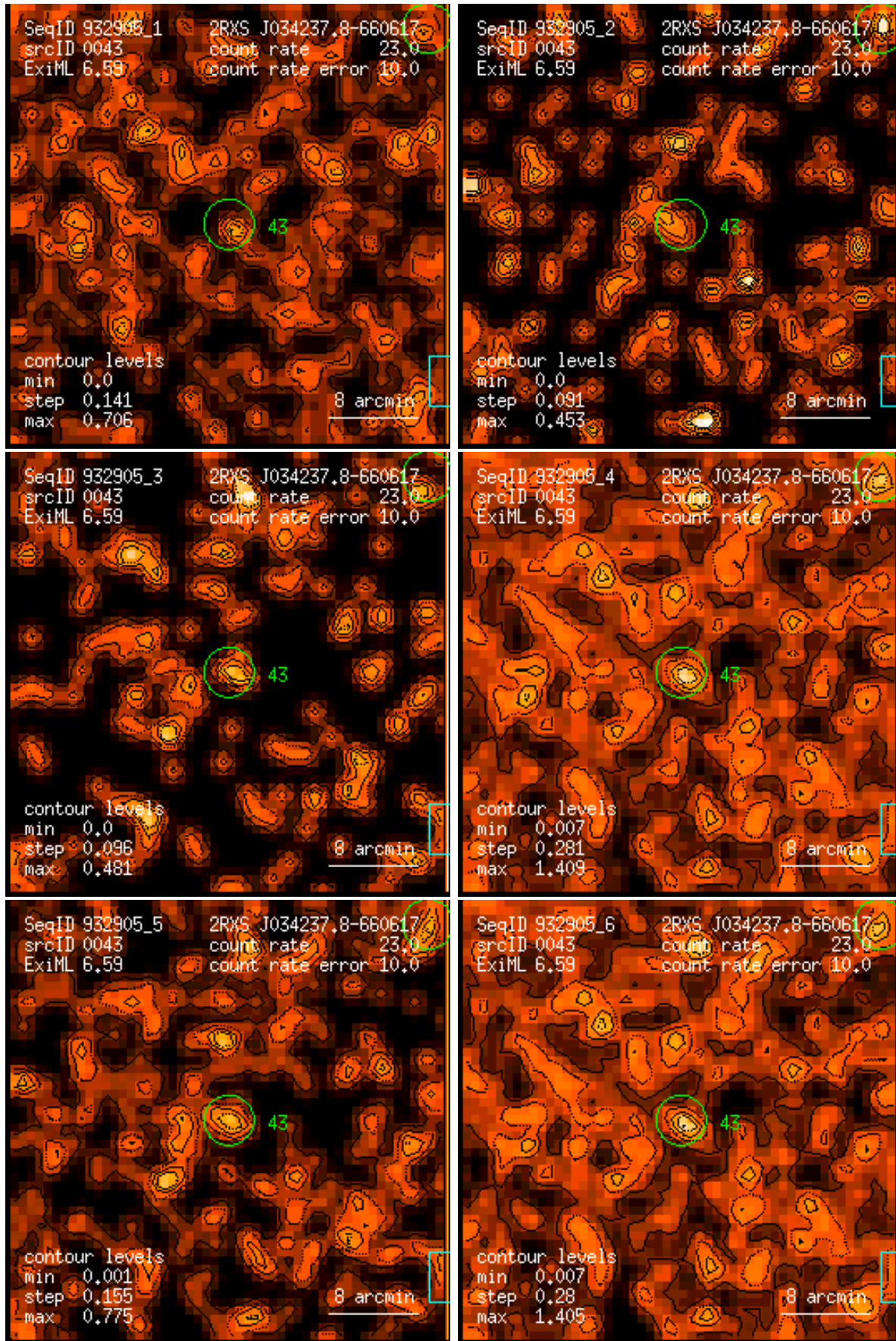
Figure 43: RASS 932905: detection 0043: band rate images, Gaussian filter: (1) PSPC channels 11 – 41, (2) 52 – 90, (3) 91 – 201, (4) 11 – 235, (5) 52 – 201, (6) 11 – 201. Broad band rates in counts/ks. Band rate contour levels in counts/ks/arcmin 2 .
