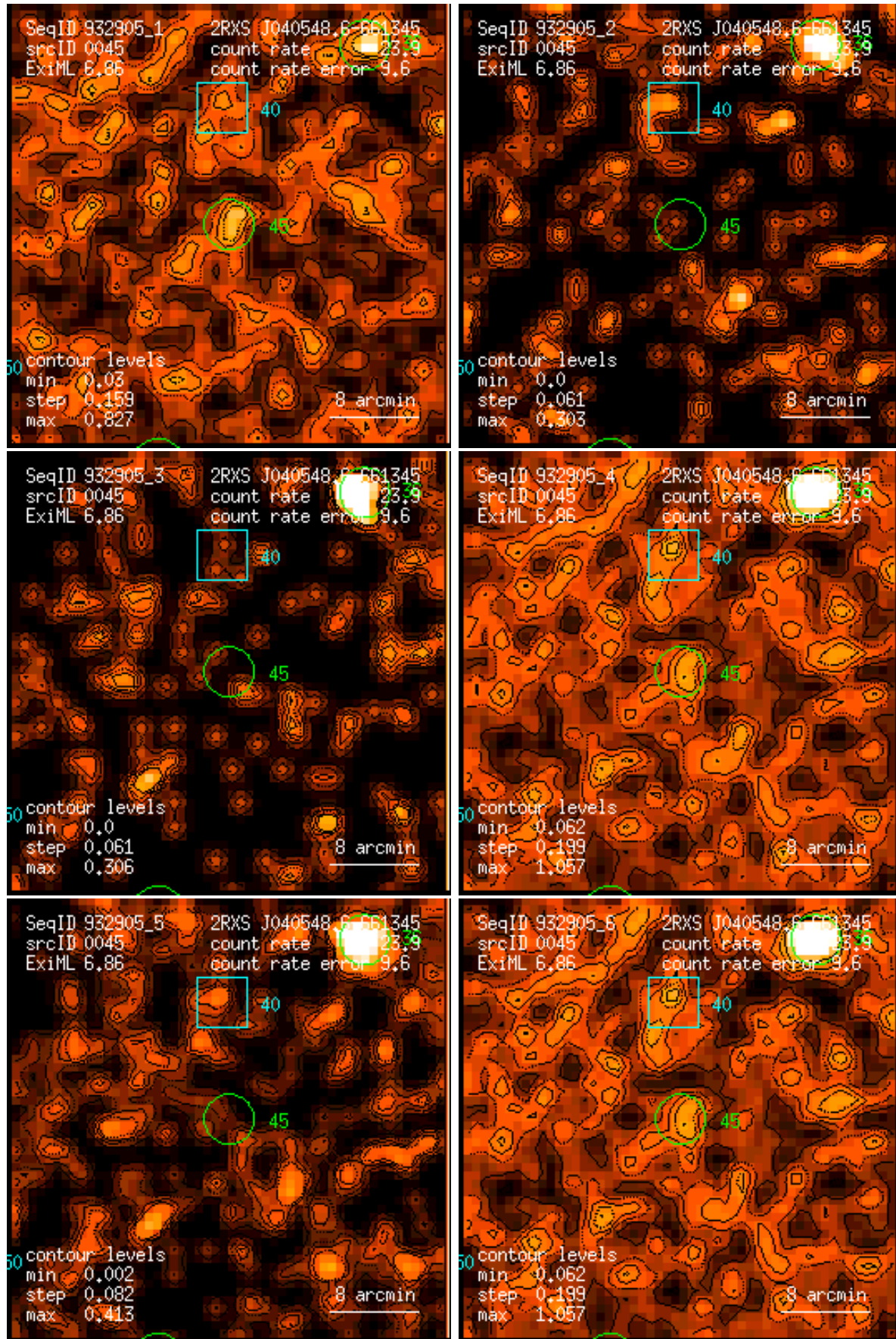
Figure 45: RASS 932905: detection 0045: band rate images, Gaussian filter: (1) PSPC channels 11 – 41, (2) 52 – 90, (3) 91 – 201, (4) 11 – 235, (5) 52 – 201, (6) 11 – 201. Broad band rates in counts/ks. Band rate contour levels in counts/ks/arcmin 2 .
