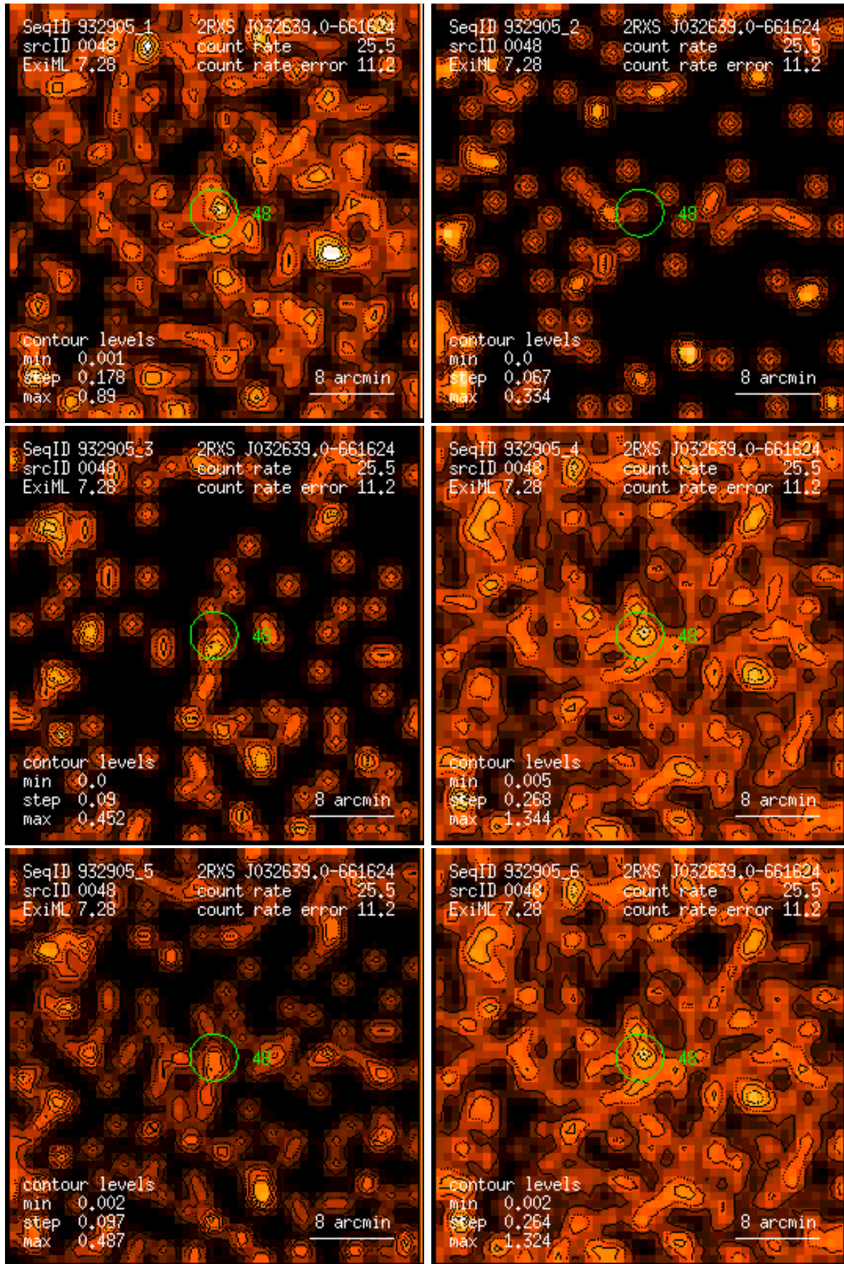
Figure 48: RASS 932905: detection 0048: band rate images, Gaussian filter: (1) PSPC channels 11 – 41, (2) 52 – 90, (3) 91 – 201, (4) 11 – 235, (5) 52 – 201, (6) 11 – 201. Broad band rates in counts/ks. Band rate contour levels in counts/ks/arcmin 2 .
