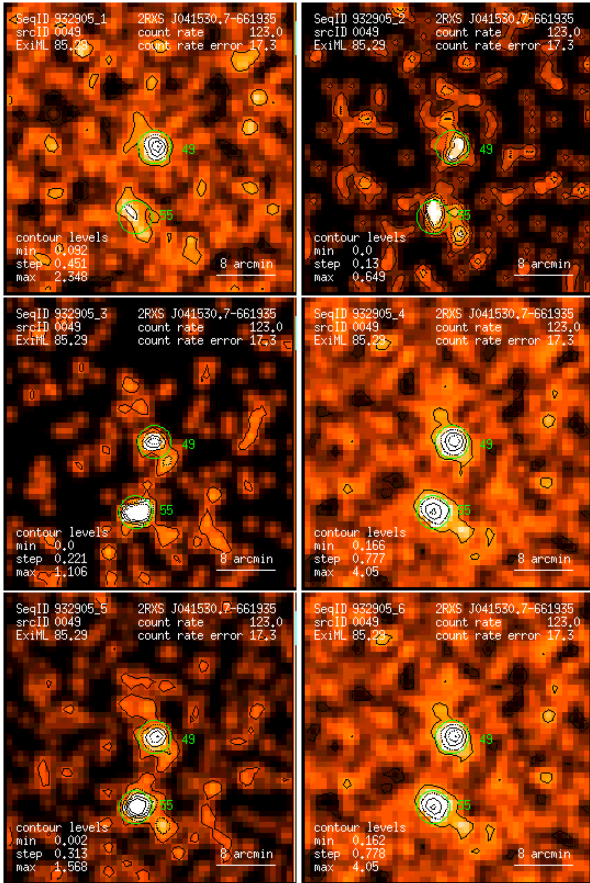
Figure 49: RASS 932905: detection 0049: band rate images, Gaussian filter: (1) PSPC channels 11 – 41, (2) 52 – 90, (3) 91 – 201, (4) 11 – 235, (5) 52 – 201, (6) 11 – 201. Broad band rates in counts/ks. Band rate contour levels in counts/ks/arcmin 2 .
