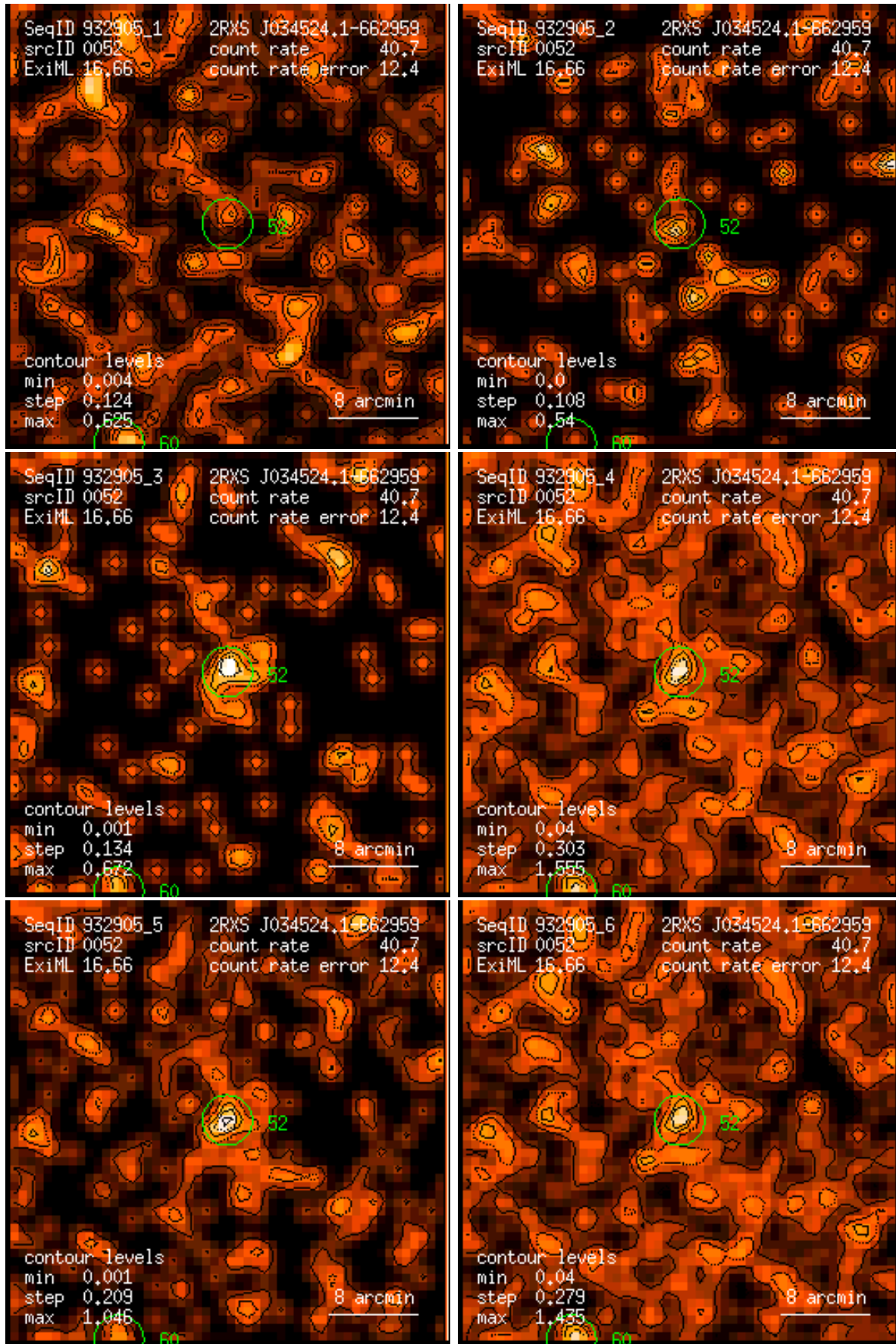
Figure 52: RASS 932905: detection 0052: band rate images, Gaussian filter: (1) PSPC channels 11 – 41, (2) 52 – 90, (3) 91 – 201, (4) 11 – 235, (5) 52 – 201, (6) 11 – 201. Broad band rates in counts/ks. Band rate contour levels in counts/ks/arcmin 2 .
