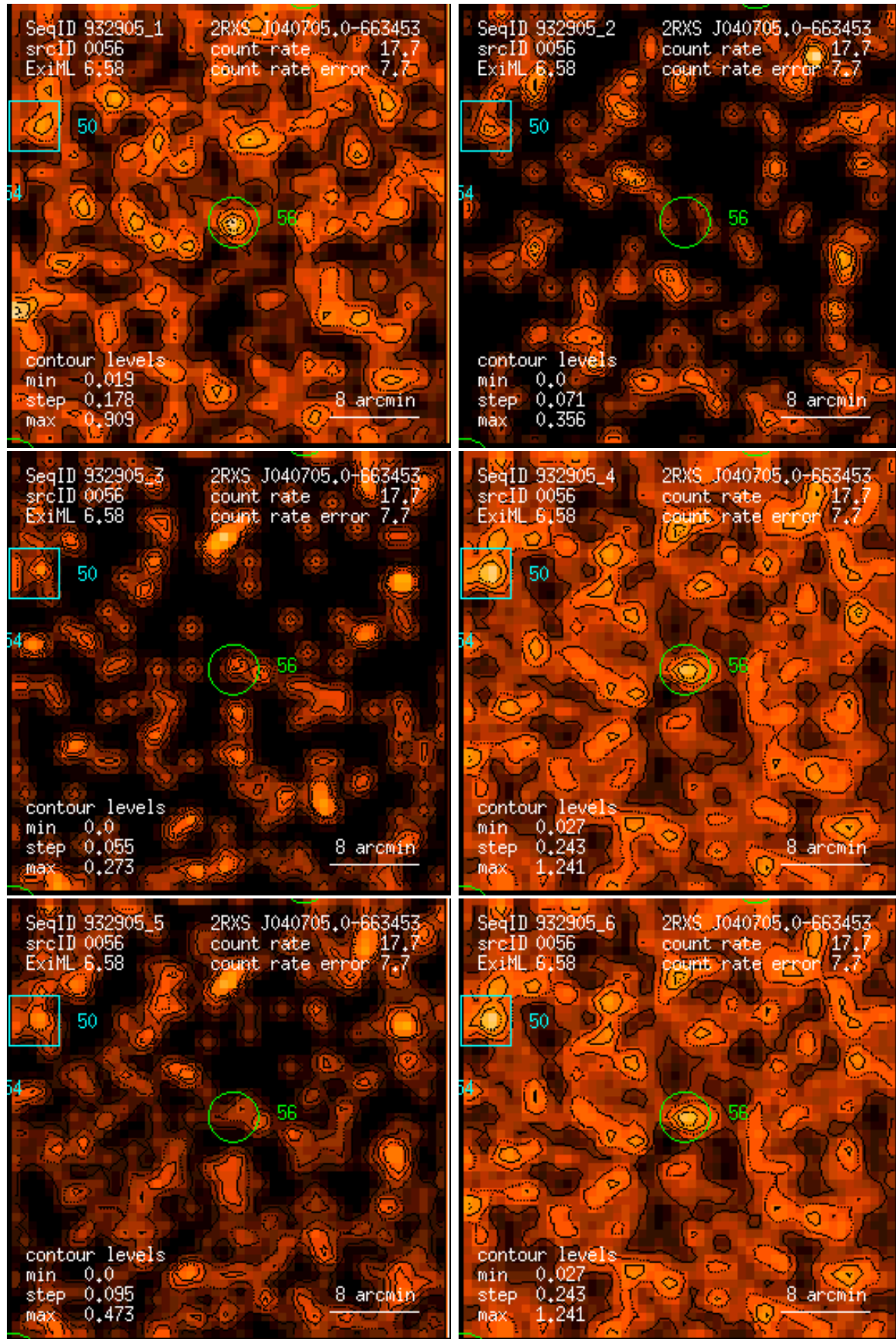
Figure 56: RASS 932905: detection 0056: band rate images, Gaussian filter: (1) PSPC channels 11 – 41, (2) 52 – 90, (3) 91 – 201, (4) 11 – 235, (5) 52 – 201, (6) 11 – 201. Broad band rates in counts/ks. Band rate contour levels in counts/ks/arcmin 2 .
