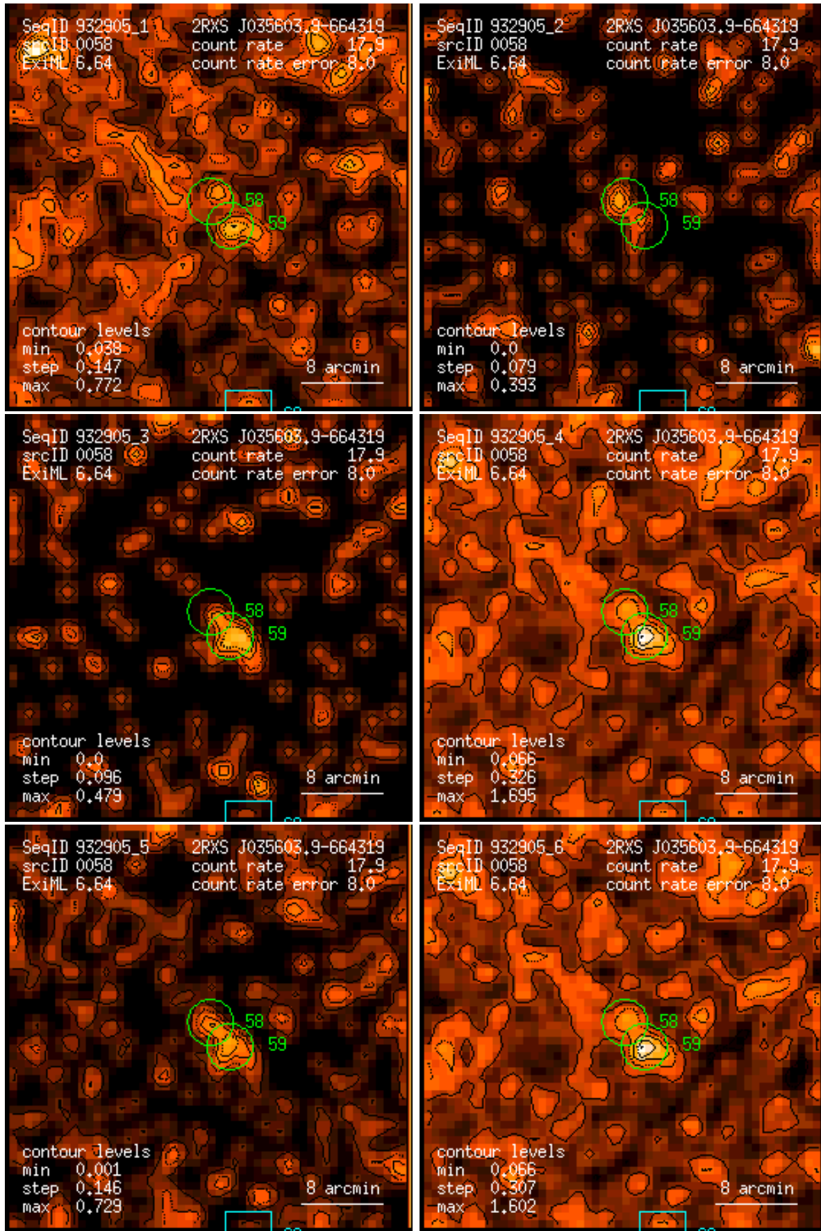
Figure 58: RASS 932905: detection 0058: band rate images, Gaussian filter: (1) PSPC channels 11 – 41, (2) 52 – 90, (3) 91 – 201, (4) 11 – 235, (5) 52 – 201, (6) 11 – 201. Broad band rates in counts/ks. Band rate contour levels in counts/ks/arcmin 2 .
