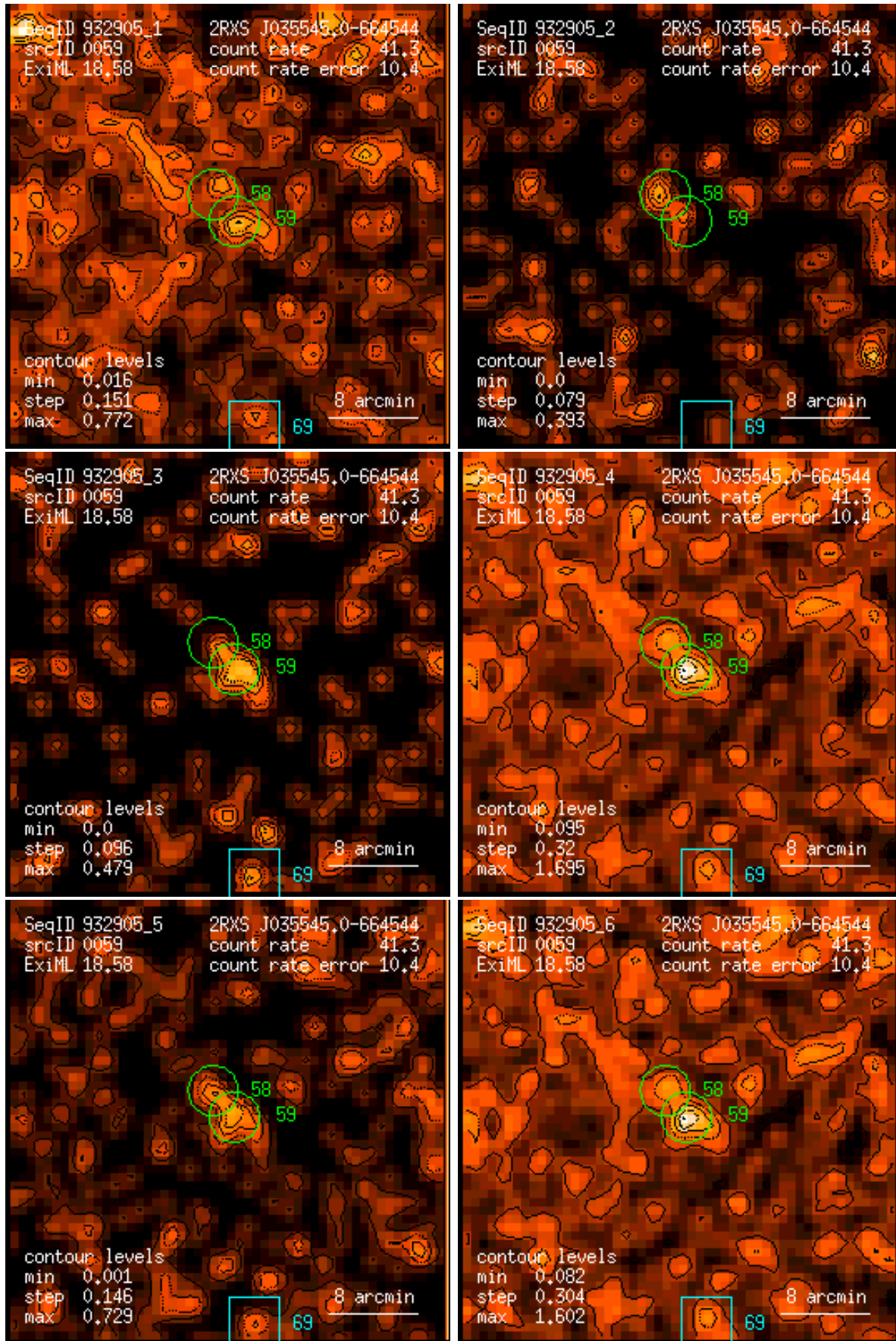
Figure 59: RASS 932905: detection 0059: band rate images, Gaussian filter: (1) PSPC channels 11 – 41, (2) 52 – 90, (3) 91 – 201, (4) 11 – 235, (5) 52 – 201, (6) 11 – 201. Broad band rates in counts/ks. Band rate contour levels in counts/ks/arcmin 2 .
