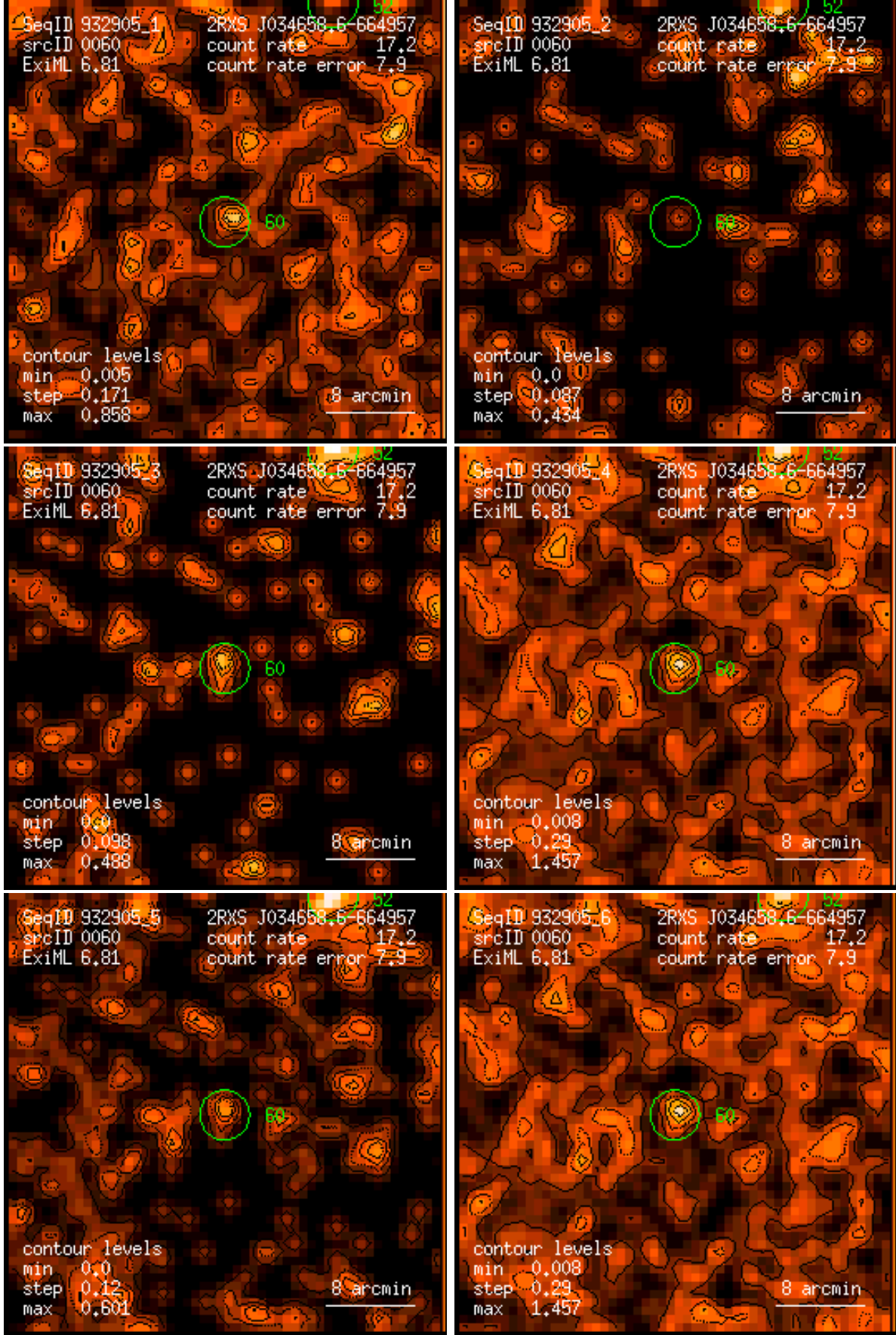
Figure 60: RASS 932905: detection 0060: band rate images, Gaussian filter: (1) PSPC channels 11 – 41, (2) 52 – 90, (3) 91 – 201, (4) 11 – 235, (5) 52 – 201, (6) 11 – 201. Broad band rates in counts/ks. Band rate contour levels in counts/ks/arcmin 2 .
