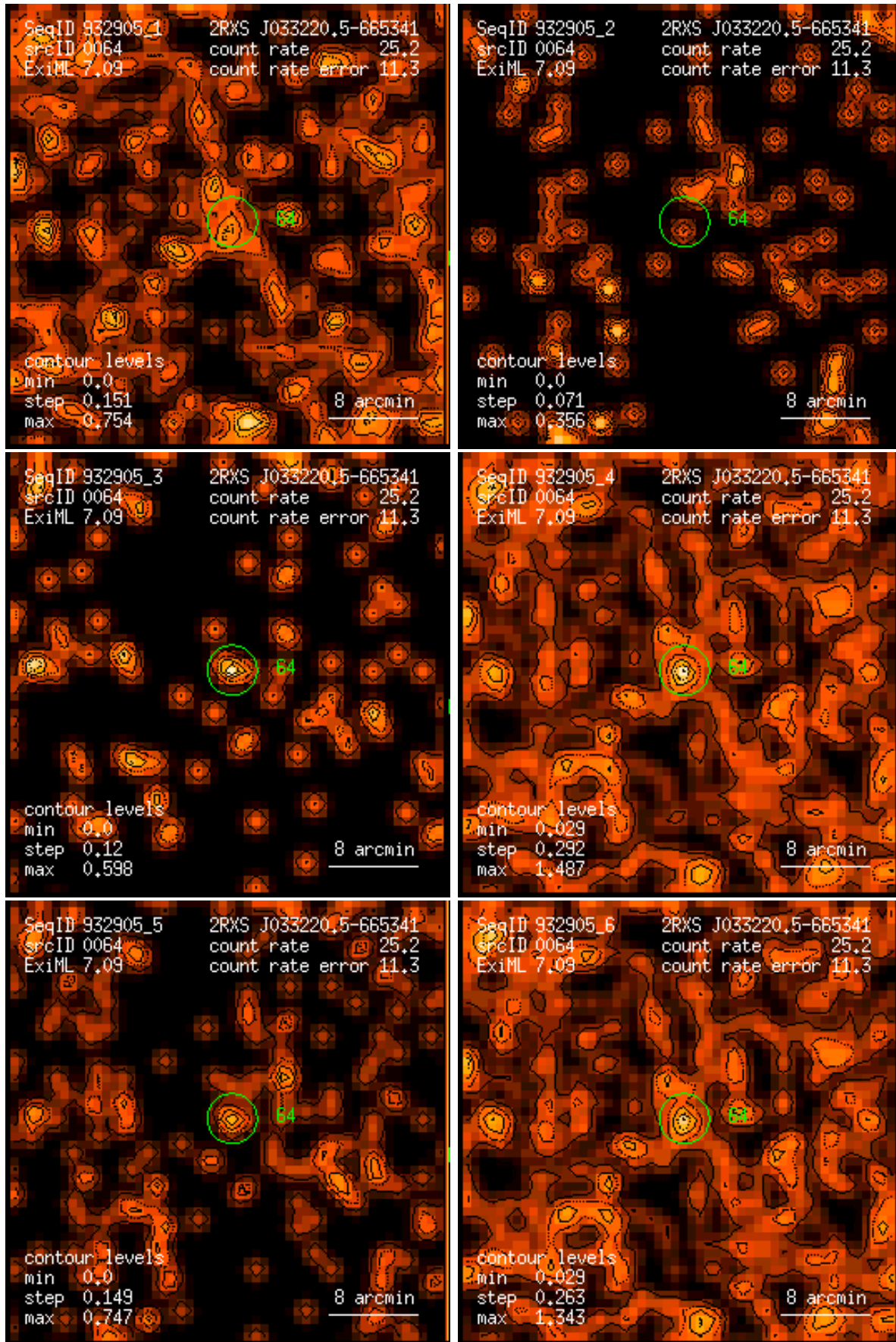
Figure 64: RASS 932905: detection 0064: band rate images, Gaussian filter: (1) PSPC channels 11 – 41, (2) 52 – 90, (3) 91 – 201, (4) 11 – 235, (5) 52 – 201, (6) 11 – 201. Broad band rates in counts/ks. Band rate contour levels in counts/ks/arcmin 2 .
