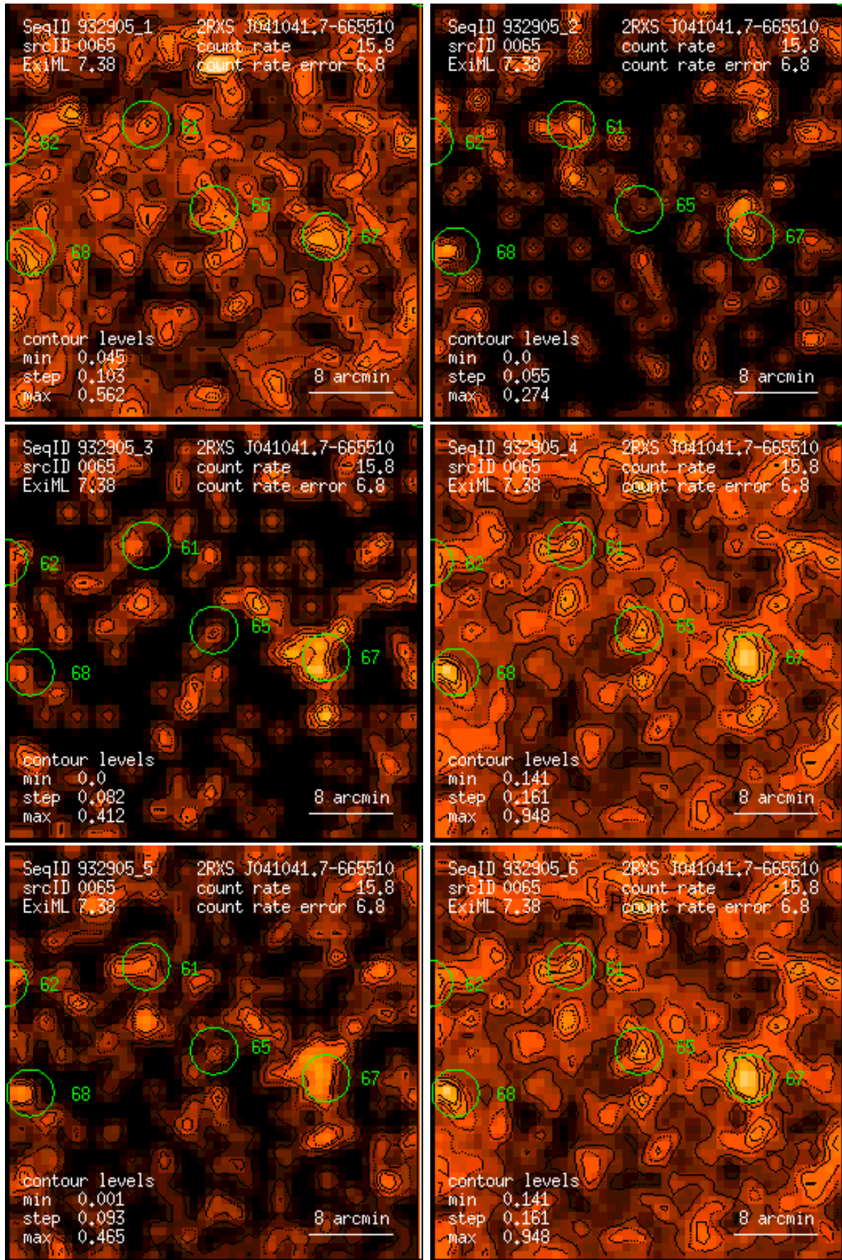
Figure 65: RASS 932905: detection 0065: band rate images, Gaussian filter: (1) PSPC channels 11 – 41, (2) 52 – 90, (3) 91 – 201, (4) 11 – 235, (5) 52 – 201, (6) 11 – 201. Broad band rates in counts/ks. Band rate contour levels in counts/ks/arcmin 2 .
