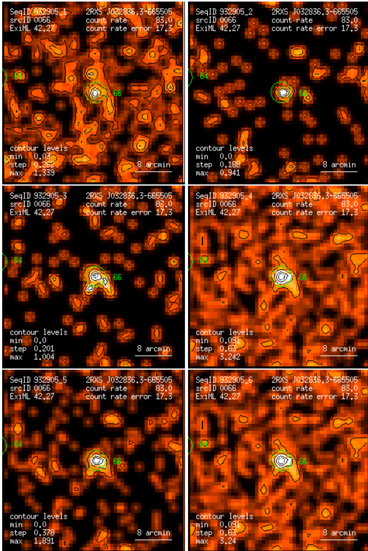
Figure 66: RASS 932905: detection 0066: band rate images, Gaussian filter: (1) PSPC channels 11 – 41, (2) 52 – 90, (3) 91 – 201, (4) 11 – 235, (5) 52 – 201, (6) 11 – 201. Broad band rates in counts/ks. Band rate contour levels in counts/ks/arcmin 2 .
