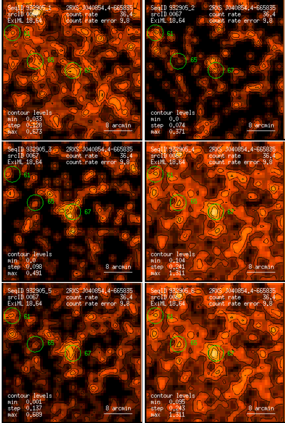
Figure 67: RASS 932905: detection 0067: band rate images, Gaussian filter: (1) PSPC channels 11 – 41, (2) 52 – 90, (3) 91 – 201, (4) 11 – 235, (5) 52 – 201, (6) 11 – 201. Broad band rates in counts/ks. Band rate contour levels in counts/ks/arcmin 2 .
