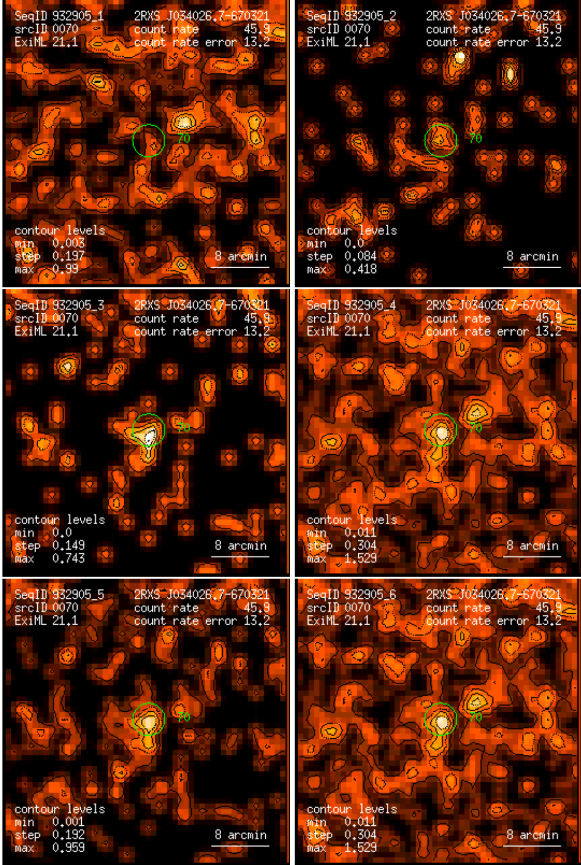
Figure 70: RASS 932905: detection 0070: band rate images, Gaussian filter: (1) PSPC channels 11 – 41, (2) 52 – 90, (3) 91 – 201, (4) 11 – 235, (5) 52 – 201, (6) 11 – 201. Broad band rates in counts/ks. Band rate contour levels in counts/ks/arcmin 2 .
