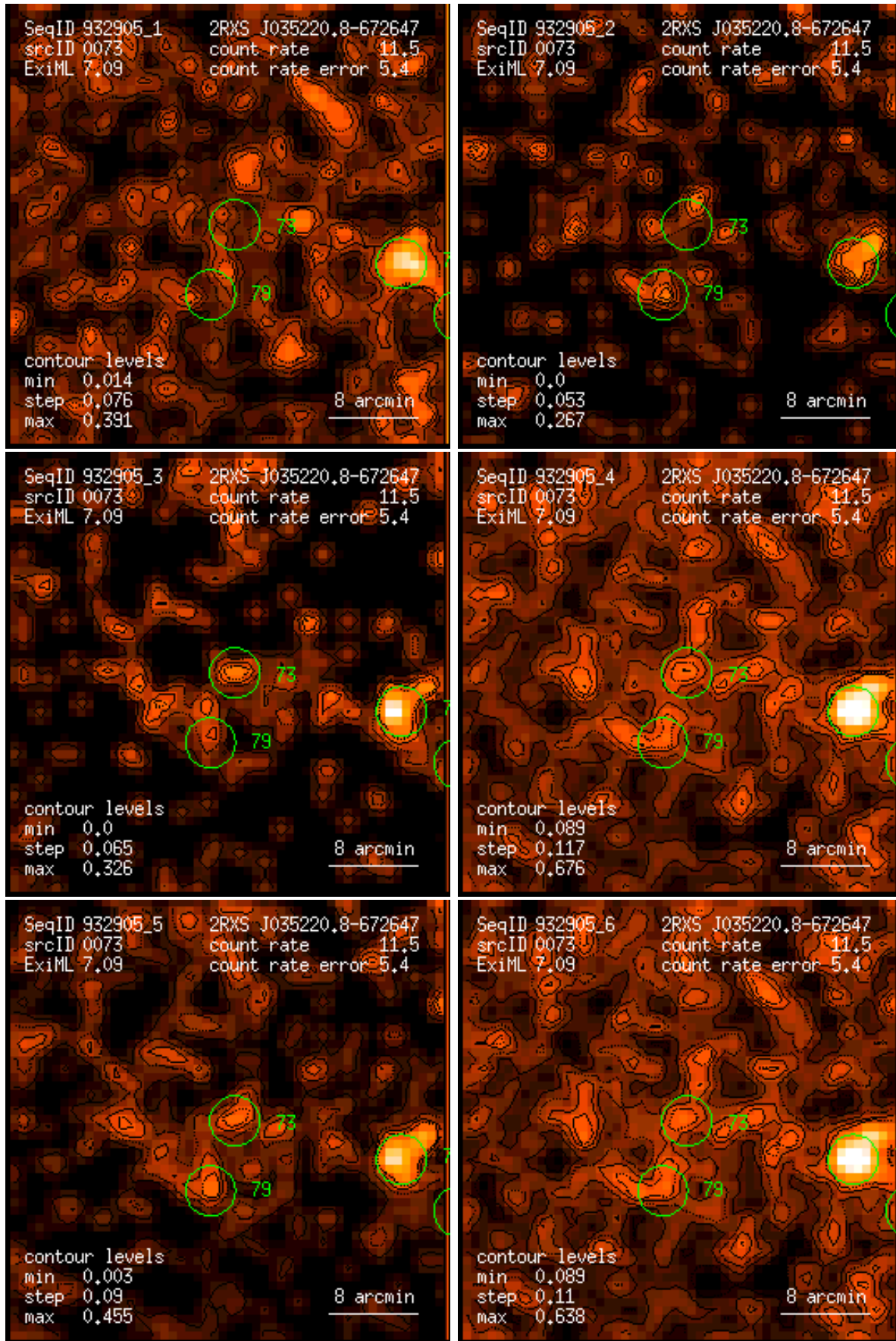
Figure 73: RASS 932905: detection 0073: band rate images, Gaussian filter: (1) PSPC channels 11 – 41, (2) 52 – 90, (3) 91 – 201, (4) 11 – 235, (5) 52 – 201, (6) 11 – 201. Broad band rates in counts/ks. Band rate contour levels in counts/ks/arcmin 2 .
