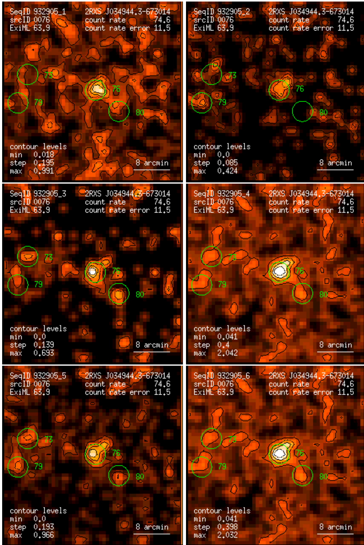
Figure 76: RASS 932905: detection 0076: band rate images, Gaussian filter: (1) PSPC channels 11 – 41, (2) 52 – 90, (3) 91 – 201, (4) 11 – 235, (5) 52 – 201, (6) 11 – 201. Broad band rates in counts/ks. Band rate contour levels in counts/ks/arcmin 2 .
