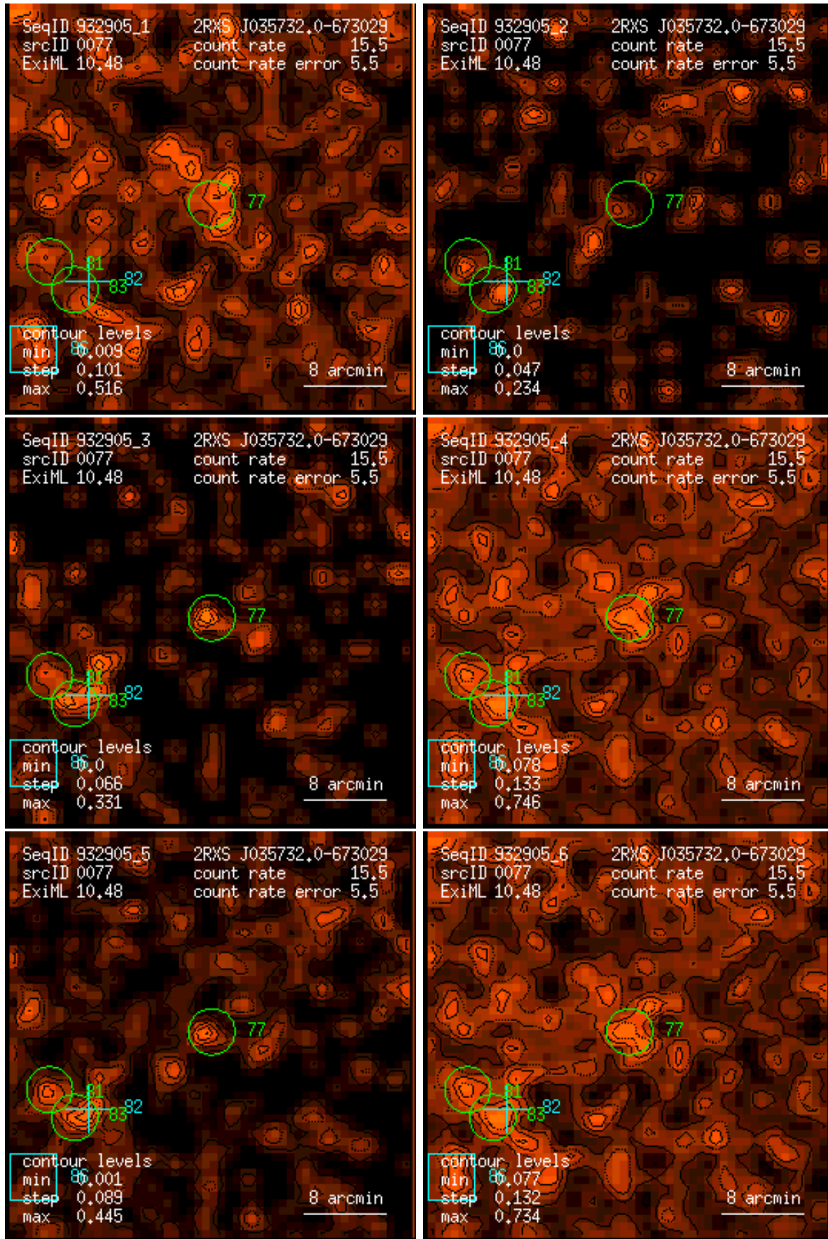
Figure 77: RASS 932905: detection 0077: band rate images, Gaussian filter: (1) PSPC channels 11 – 41, (2) 52 – 90, (3) 91 – 201, (4) 11 – 235, (5) 52 – 201, (6) 11 – 201. Broad band rates in counts/ks. Band rate contour levels in counts/ks/arcmin 2 .
