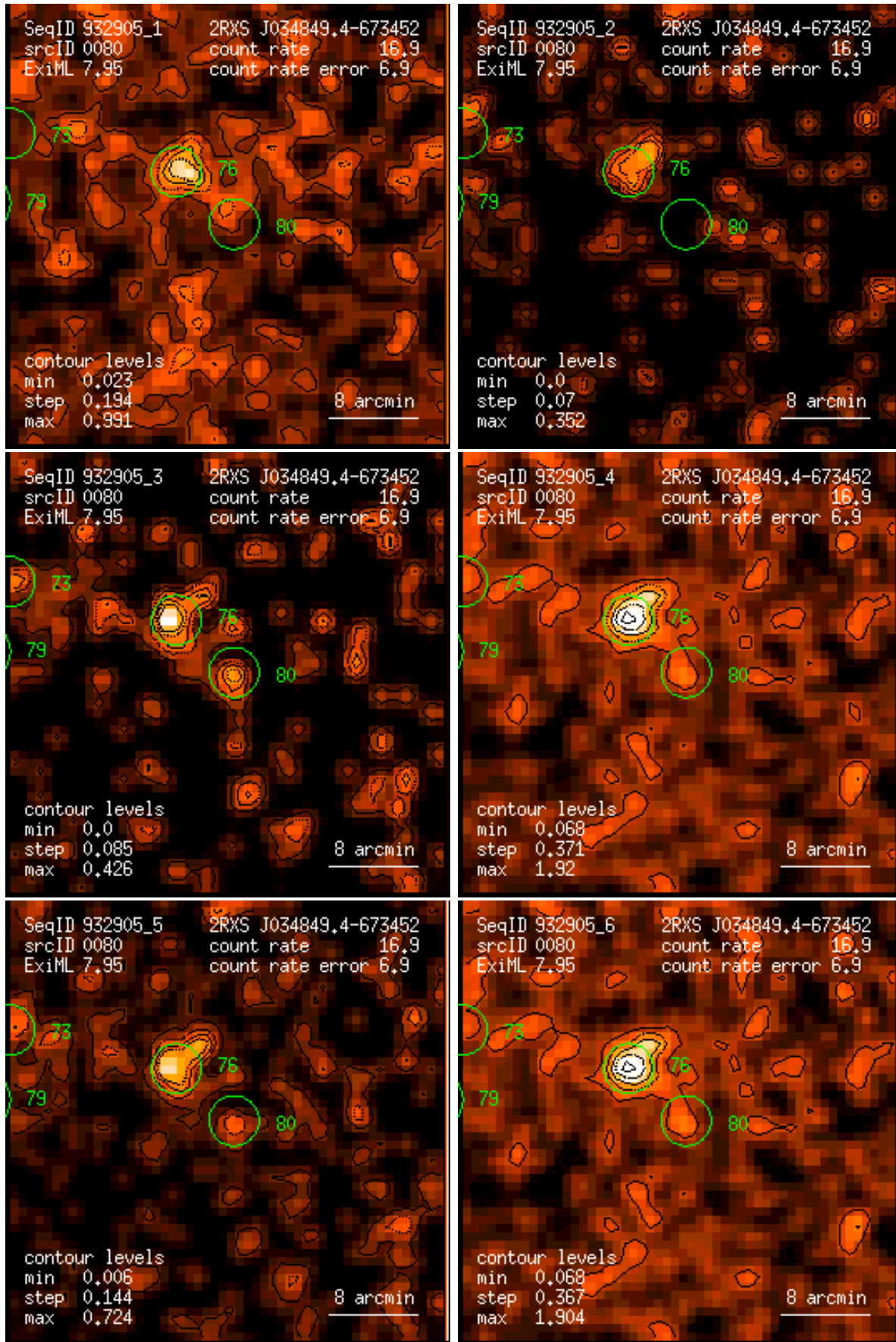
Figure 80: RASS 932905: detection 0080: band rate images, Gaussian filter: (1) PSPC channels 11 – 41, (2) 52 – 90, (3) 91 – 201, (4) 11 – 235, (5) 52 – 201, (6) 11 – 201. Broad band rates in counts/ks. Band rate contour levels in counts/ks/arcmin 2 .
