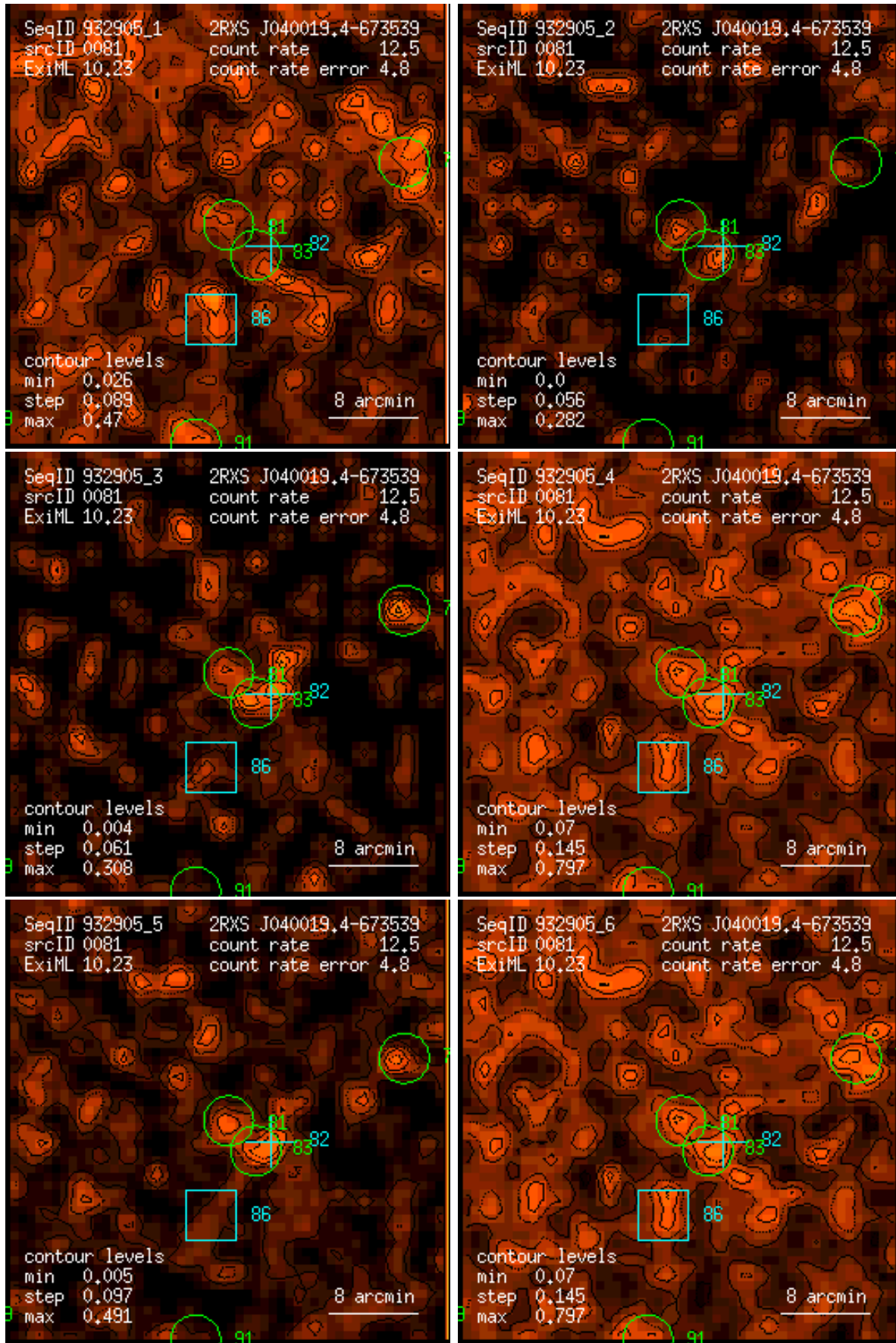
Figure 81: RASS 932905: detection 0081: band rate images, Gaussian filter: (1) PSPC channels 11 – 41, (2) 52 – 90, (3) 91 – 201, (4) 11 – 235, (5) 52 – 201, (6) 11 – 201. Broad band rates in counts/ks. Band rate contour levels in counts/ks/arcmin 2 .
