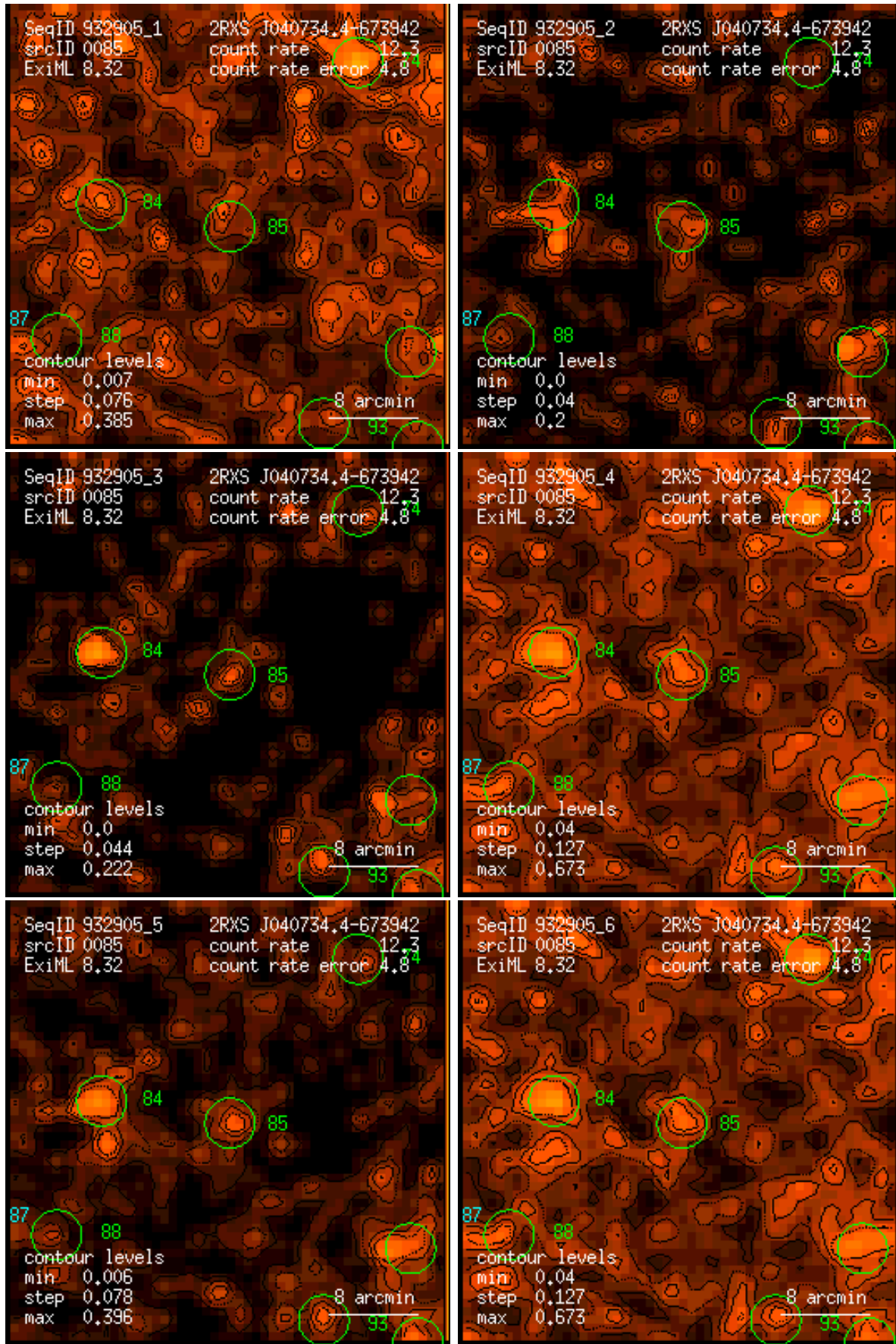
Figure 85: RASS 932905: detection 0085: band rate images, Gaussian filter: (1) PSPC channels 11 – 41, (2) 52 – 90, (3) 91 – 201, (4) 11 – 235, (5) 52 – 201, (6) 11 – 201. Broad band rates in counts/ks. Band rate contour levels in counts/ks/arcmin 2 .
