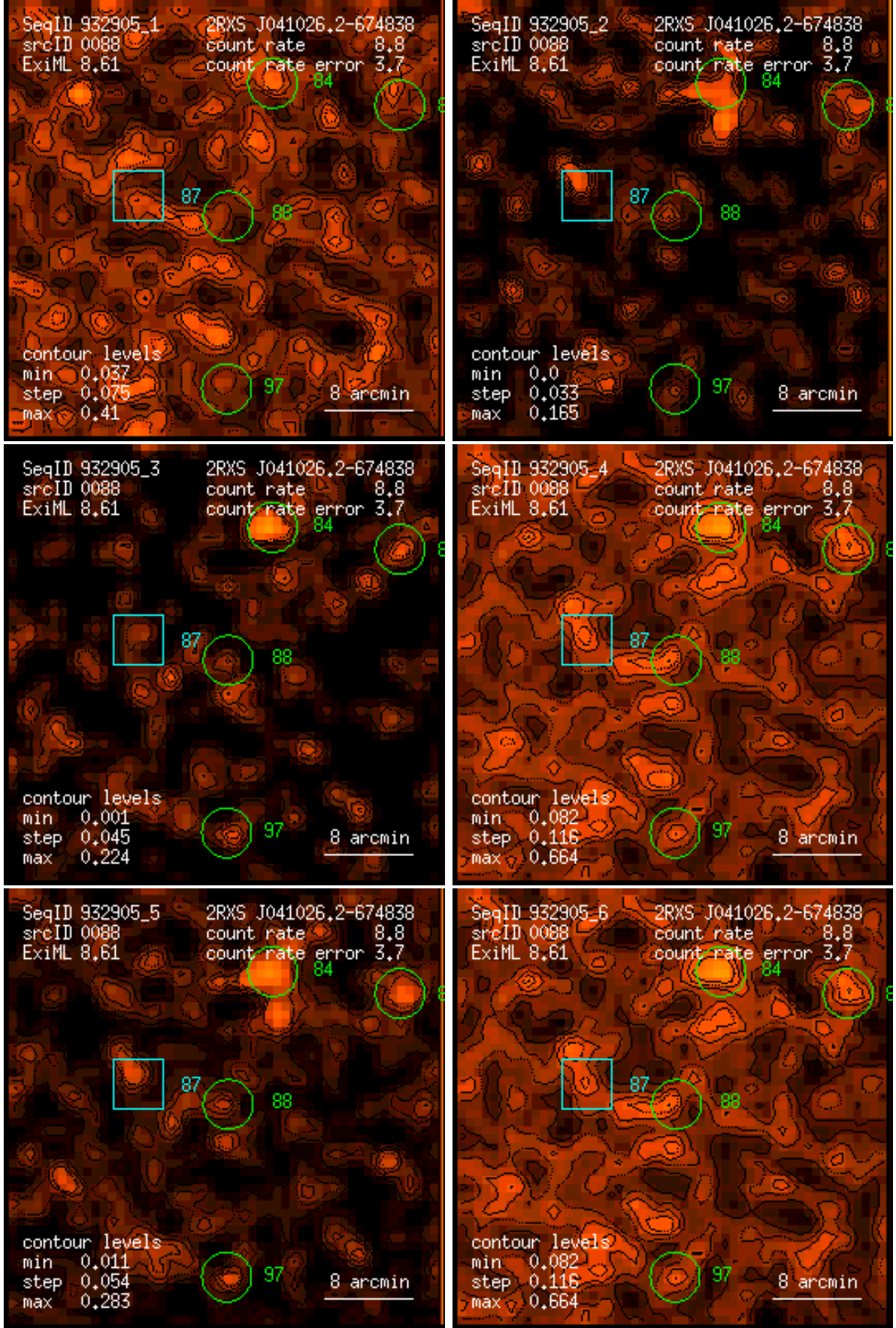
Figure 88: RASS 932905: detection 0088: band rate images, Gaussian filter: (1) PSPC channels 11 – 41, (2) 52 – 90, (3) 91 – 201, (4) 11 – 235, (5) 52 – 201, (6) 11 – 201. Broad band rates in counts/ks. Band rate contour levels in counts/ks/arcmin 2 .
