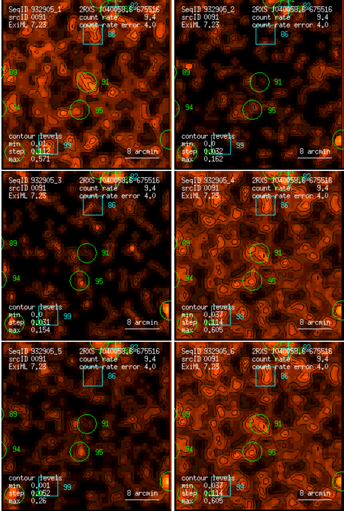
Figure 91: RASS 932905: detection 0091: band rate images, Gaussian filter: (1) PSPC channels 11 – 41, (2) 52 – 90, (3) 91 – 201, (4) 11 – 235, (5) 52 – 201, (6) 11 – 201. Broad band rates in counts/ks. Band rate contour levels in counts/ks/arcmin 2 .
