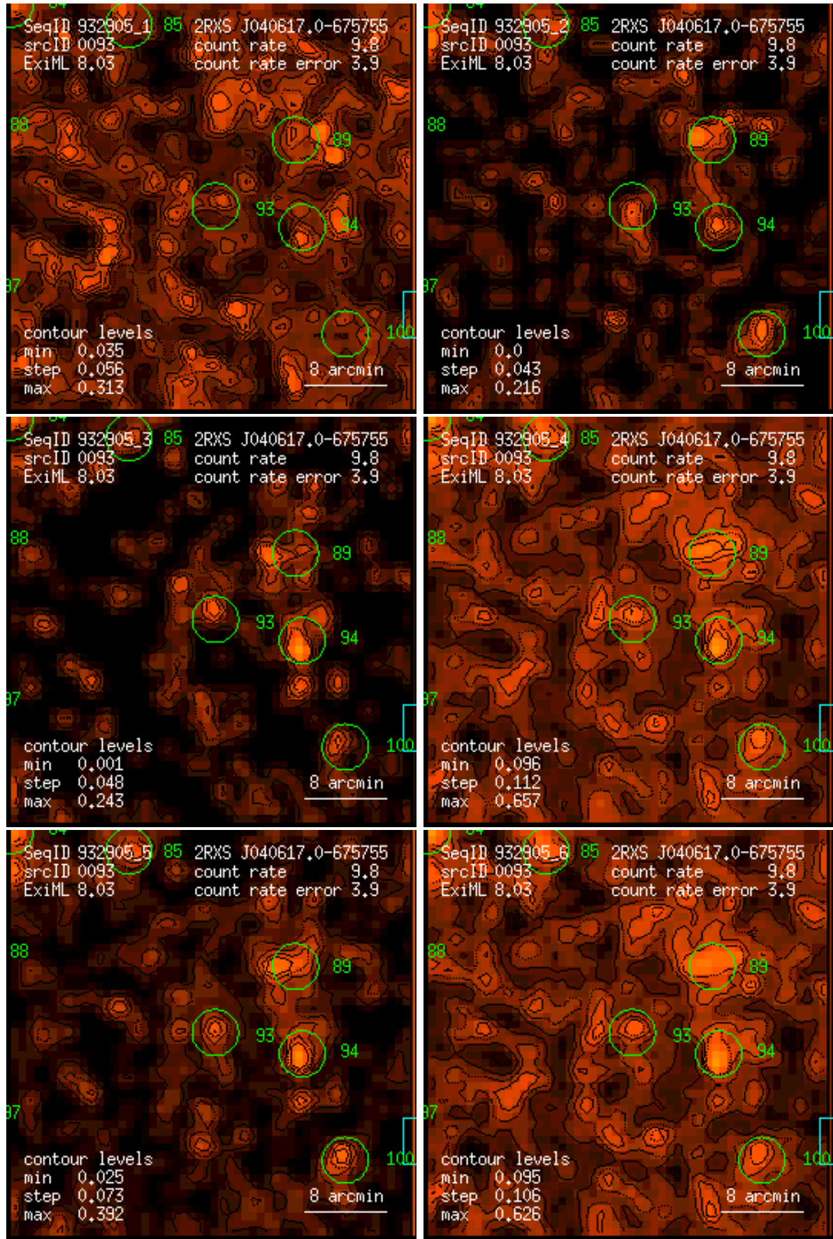
Figure 93: RASS 932905: detection 0093: band rate images, Gaussian filter: (1) PSPC channels 11 – 41, (2) 52 – 90, (3) 91 – 201, (4) 11 – 235, (5) 52 – 201, (6) 11 – 201. Broad band rates in counts/ks. Band rate contour levels in counts/ks/arcmin 2 .
