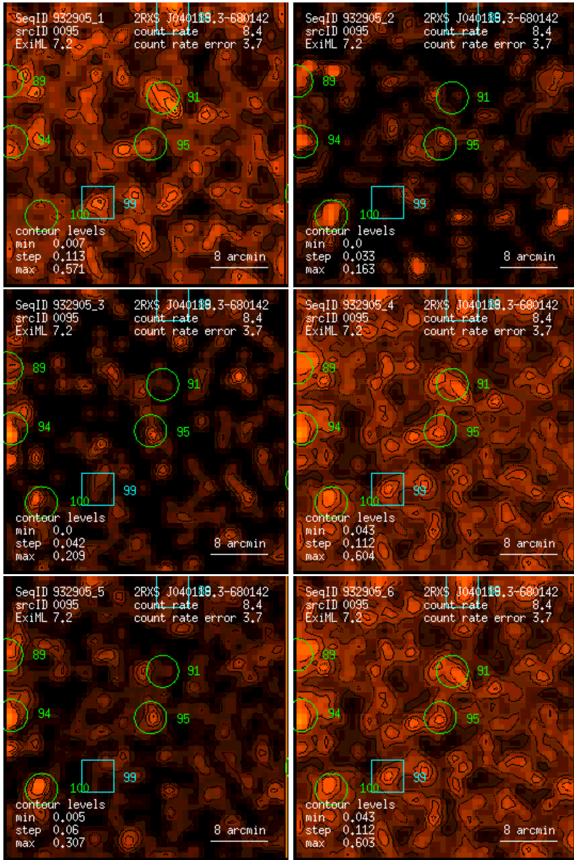
Figure 95: RASS 932905: detection 0095: band rate images, Gaussian filter: (1) PSPC channels 11 – 41, (2) 52 – 90, (3) 91 – 201, (4) 11 – 235, (5) 52 – 201, (6) 11 – 201. Broad band rates in counts/ks. Band rate contour levels in counts/ks/arcmin 2 .
