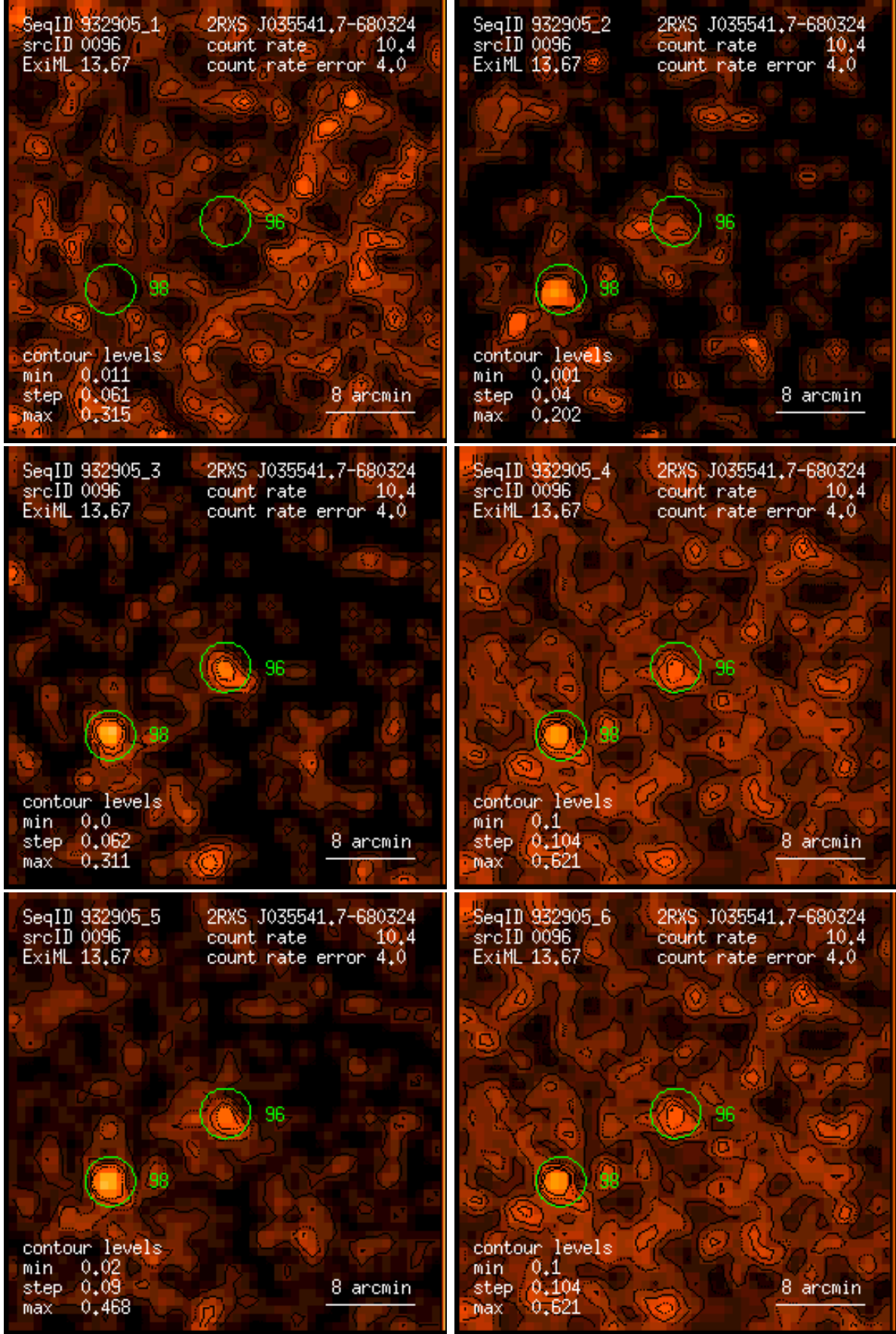
Figure 96: RASS 932905: detection 0096: band rate images, Gaussian filter: (1) PSPC channels 11 – 41, (2) 52 – 90, (3) 91 – 201, (4) 11 – 235, (5) 52 – 201, (6) 11 – 201. Broad band rates in counts/ks. Band rate contour levels in counts/ks/arcmin 2 .
