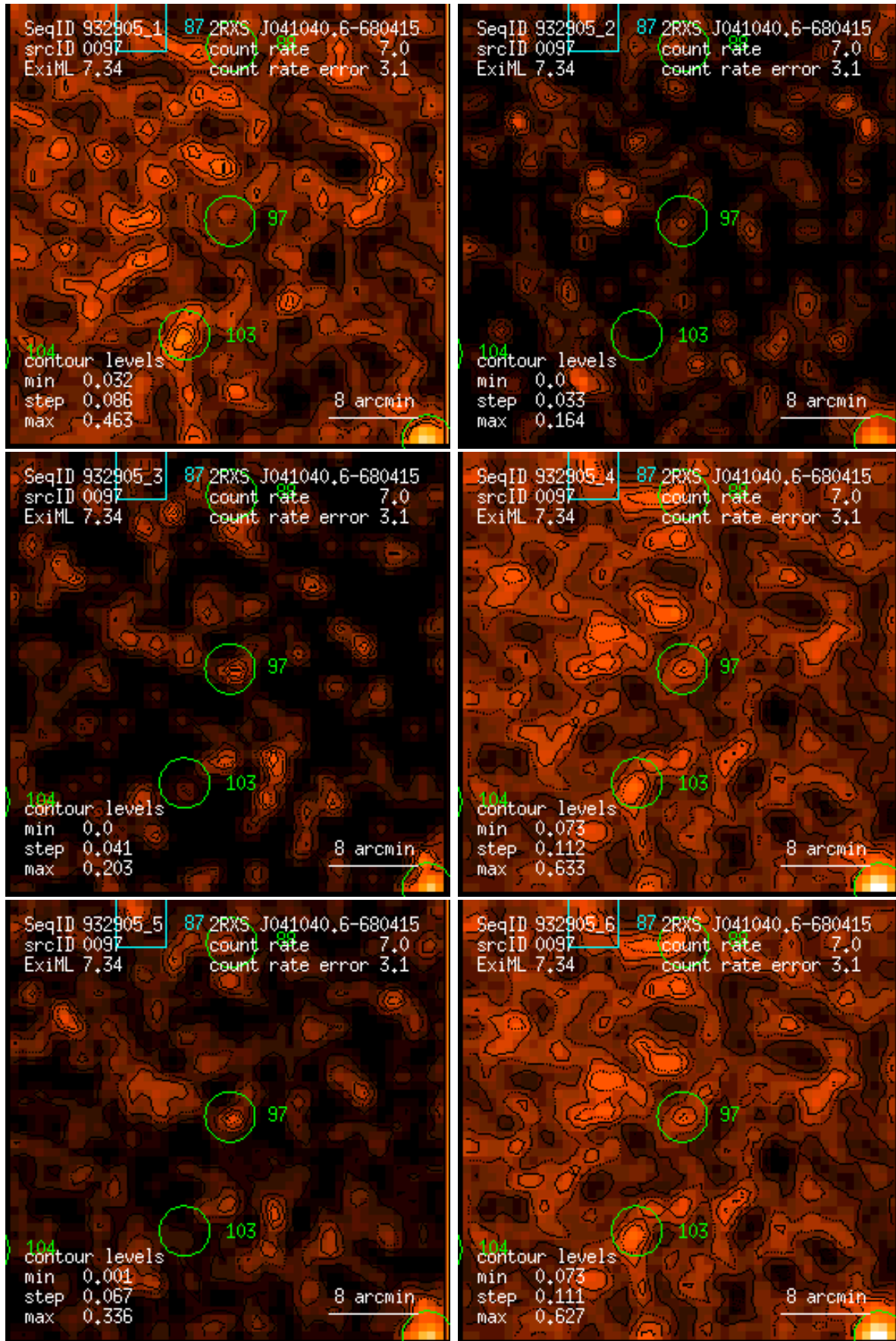
Figure 97: RASS 932905: detection 0097: band rate images, Gaussian filter: (1) PSPC channels 11 – 41, (2) 52 – 90, (3) 91 – 201, (4) 11 – 235, (5) 52 – 201, (6) 11 – 201. Broad band rates in counts/ks. Band rate contour levels in counts/ks/arcmin 2 .
