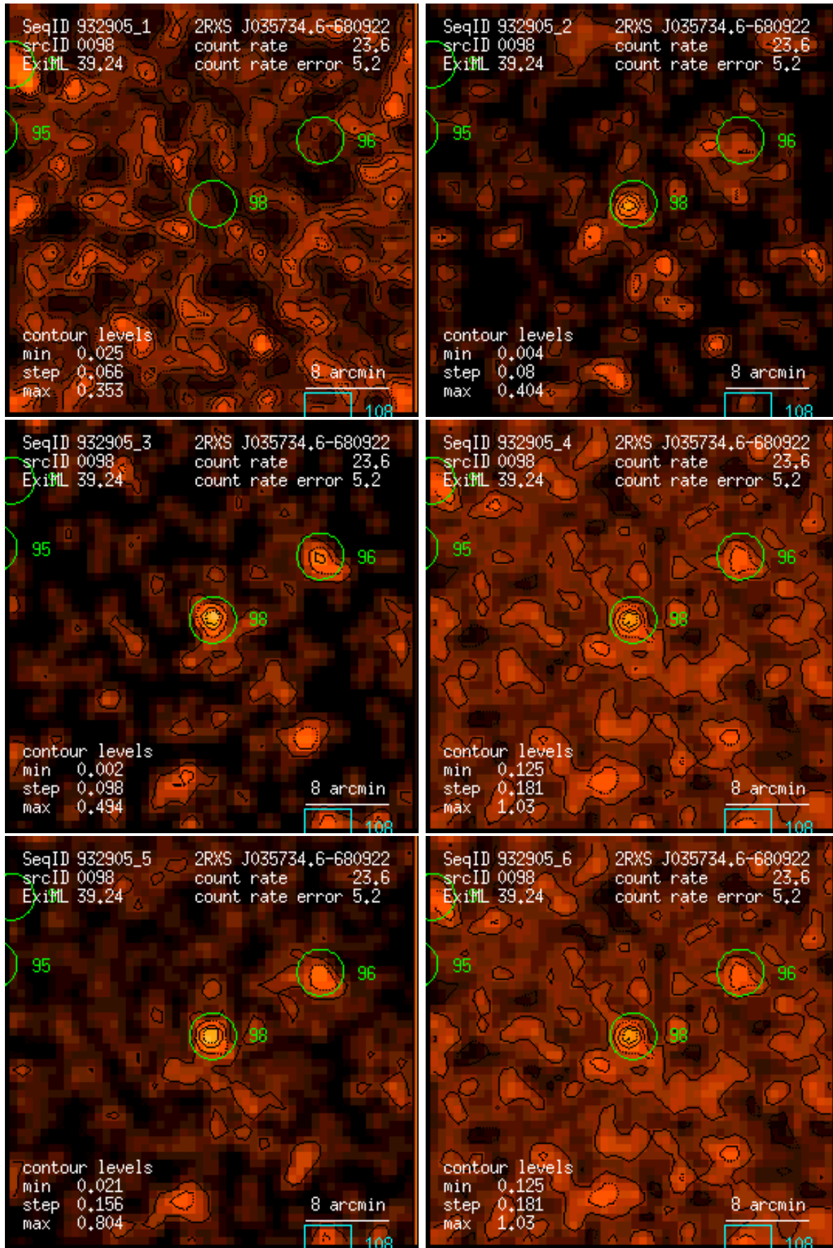
Figure 98: RASS 932905: detection 0098: band rate images, Gaussian filter: (1) PSPC channels 11 – 41, (2) 52 – 90, (3) 91 – 201, (4) 11 – 235, (5) 52 – 201, (6) 11 – 201. Broad band rates in counts/ks. Band rate contour levels in counts/ks/arcmin 2 .
