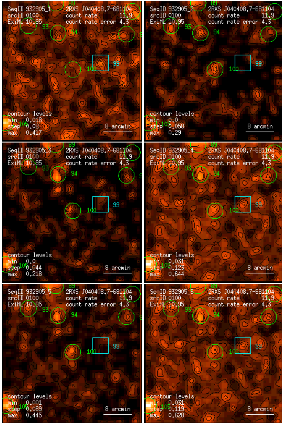
Figure 100: RASS 932905: detection 0100: band rate images, Gaussian filter: (1) PSPC channels 11 – 41, (2) 52 – 90, (3) 91 – 201, (4) 11 – 235, (5) 52 – 201, (6) 11 – 201. Broad band rates in counts/ks. Band rate contour levels in counts/ks/arcmin 2 .
