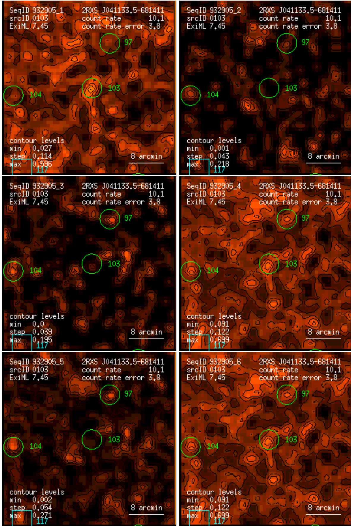
Figure 103: RASS 932905: detection 0103: band rate images, Gaussian filter: (1) PSPC channels 11 – 41, (2) 52 – 90, (3) 91 – 201, (4) 11 – 235, (5) 52 – 201, (6) 11 – 201. Broad band rates in counts/ks. Band rate contour levels in counts/ks/arcmin 2 .
