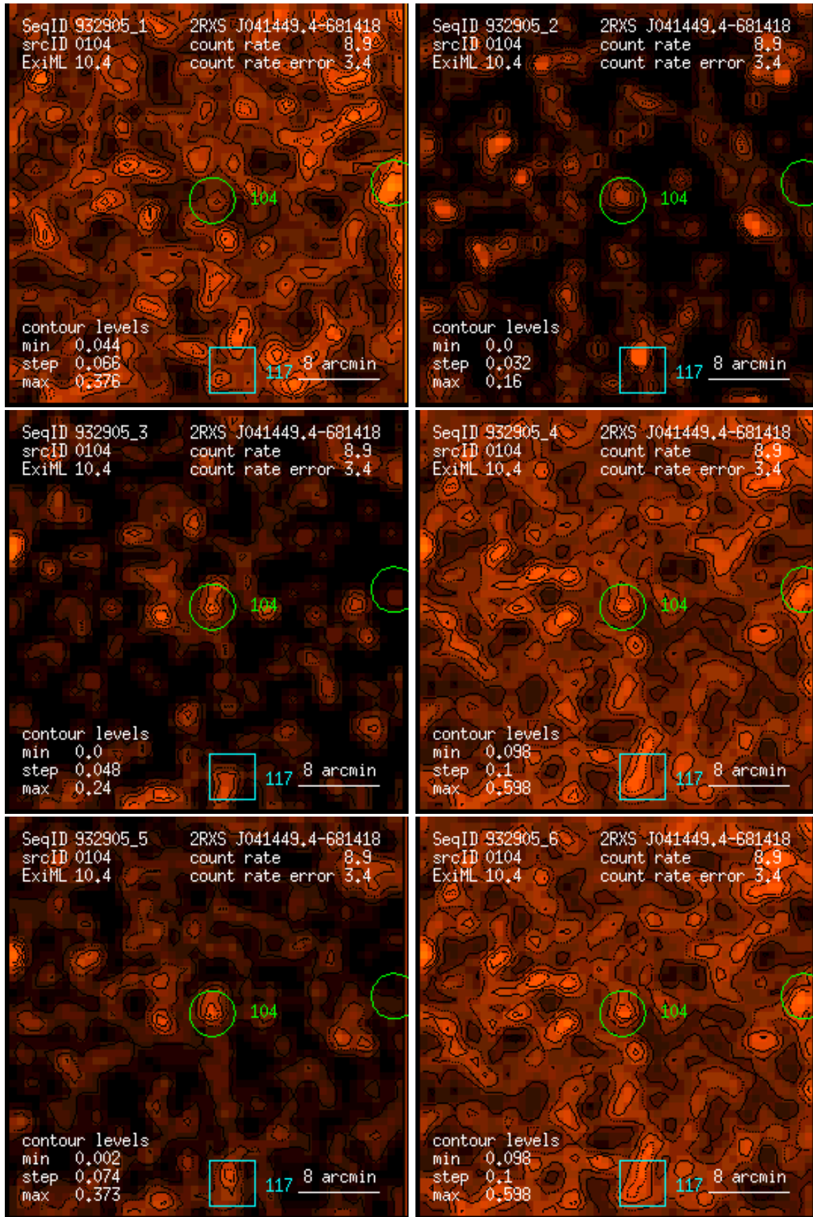
Figure 104: RASS 932905: detection 0104: band rate images, Gaussian filter: (1) PSPC channels 11 – 41, (2) 52 – 90, (3) 91 – 201, (4) 11 – 235, (5) 52 – 201, (6) 11 – 201. Broad band rates in counts/ks. Band rate contour levels in counts/ks/arcmin 2 .
