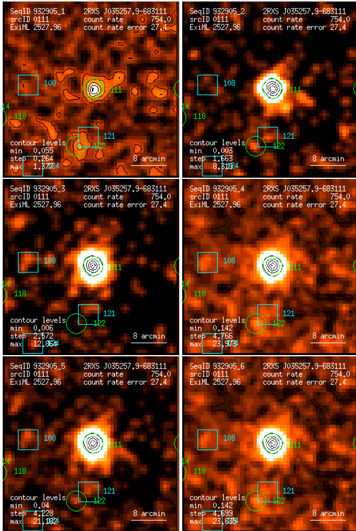
Figure 111: RASS 932905: detection 0111: band rate images, Gaussian filter: (1) PSPC channels 11 – 41, (2) 52 – 90, (3) 91 – 201, (4) 11 – 235, (5) 52 – 201, (6) 11 – 201. Broad band rates in counts/ks. Band rate contour levels in counts/ks/arcmin 2 .
