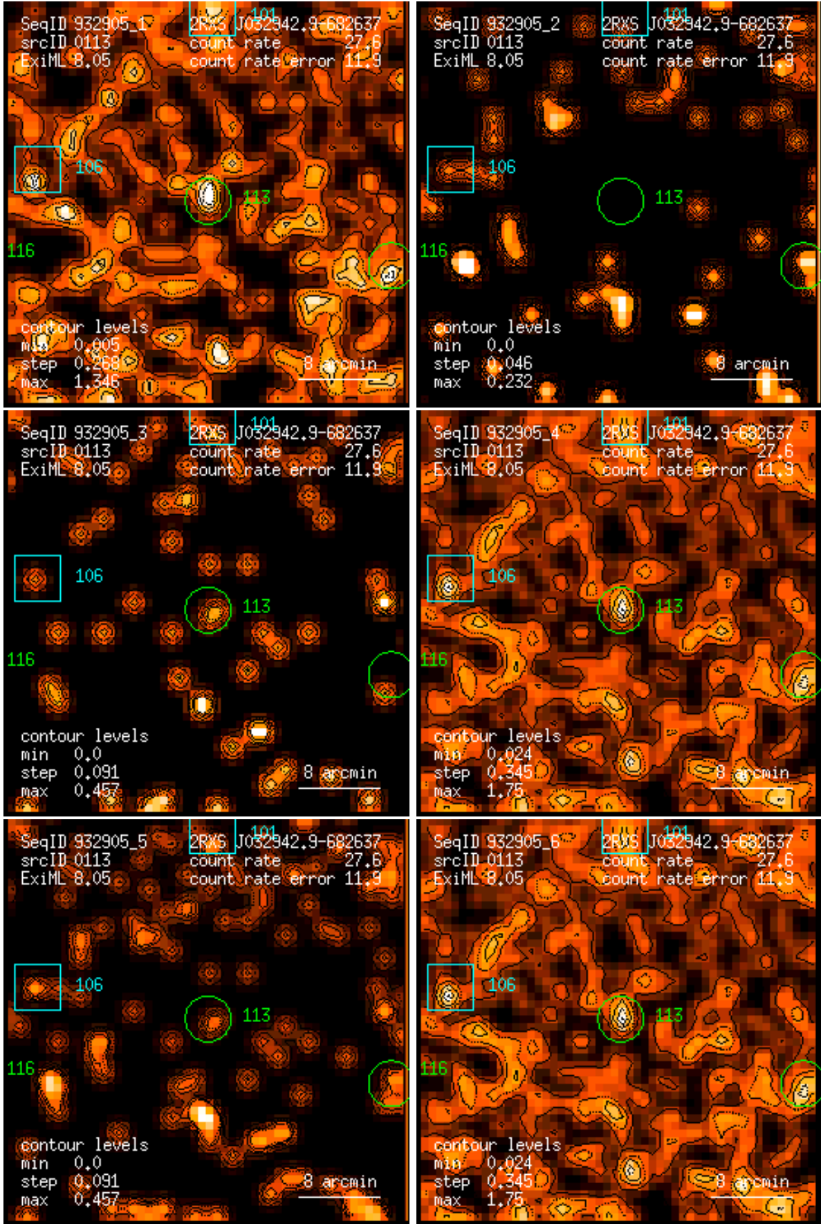
Figure 113: RASS 932905: detection 0113: band rate images, Gaussian filter: (1) PSPC channels 11 – 41, (2) 52 – 90, (3) 91 – 201, (4) 11 – 235, (5) 52 – 201, (6) 11 – 201. Broad band rates in counts/ks. Band rate contour levels in counts/ks/arcmin 2 .
