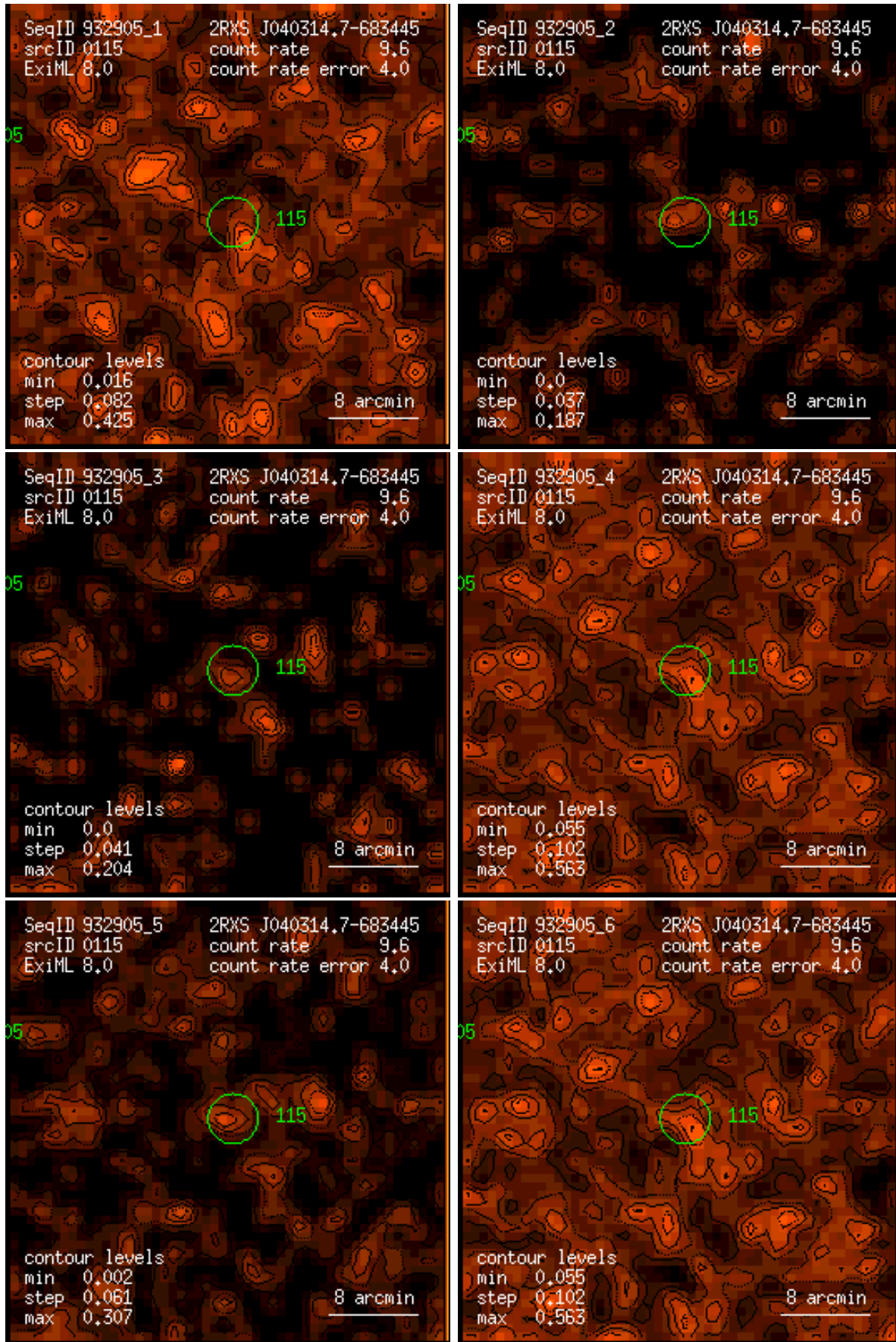
Figure 115: RASS 932905: detection 0115: band rate images, Gaussian filter: (1) PSPC channels 11 – 41, (2) 52 – 90, (3) 91 – 201, (4) 11 – 235, (5) 52 – 201, (6) 11 – 201. Broad band rates in counts/ks. Band rate contour levels in counts/ks/arcmin 2 .
