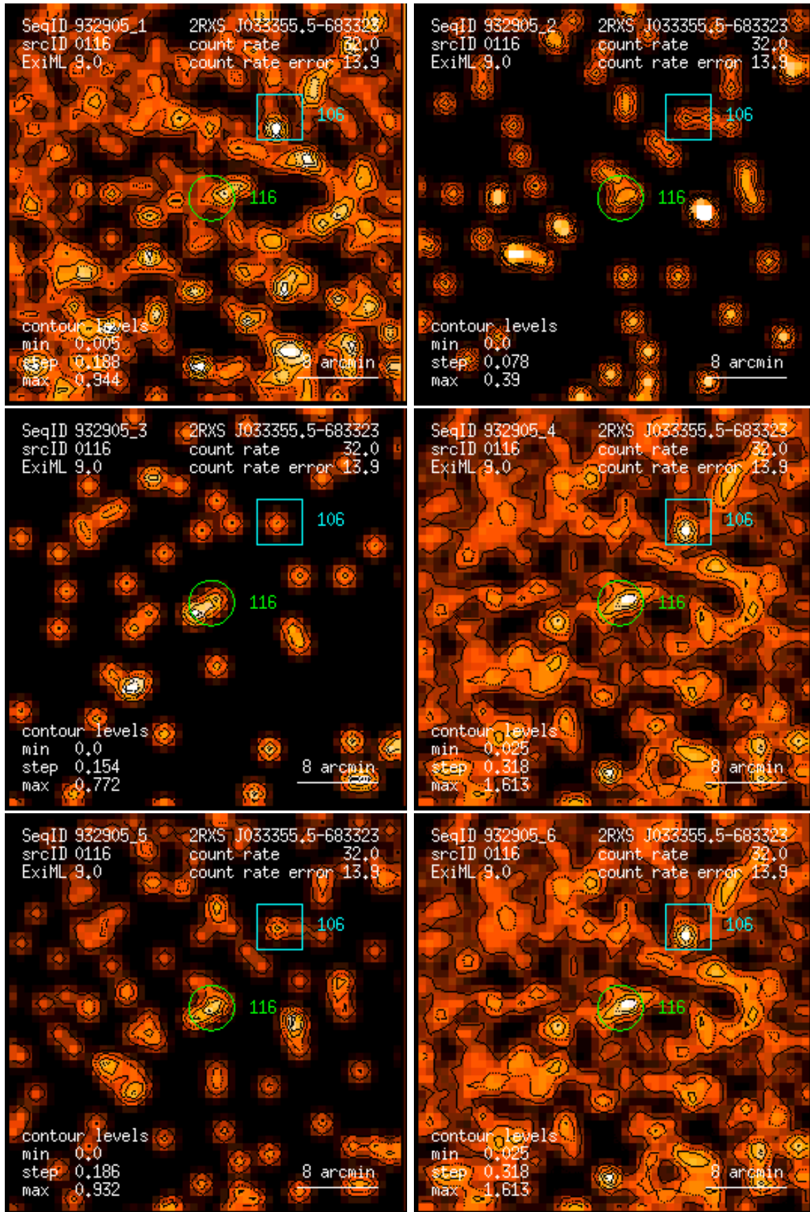
Figure 116: RASS 932905: detection 0116: band rate images, Gaussian filter: (1) PSPC channels 11 – 41, (2) 52 – 90, (3) 91 – 201, (4) 11 – 235, (5) 52 – 201, (6) 11 – 201. Broad band rates in counts/ks. Band rate contour levels in counts/ks/arcmin 2 .
